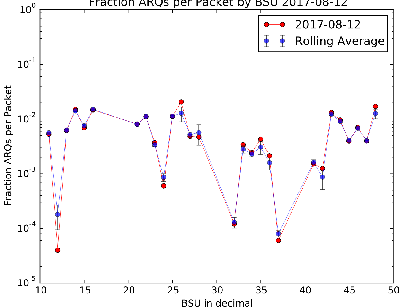
Fraction ARQs per Packet by BSU 2017-08-12
