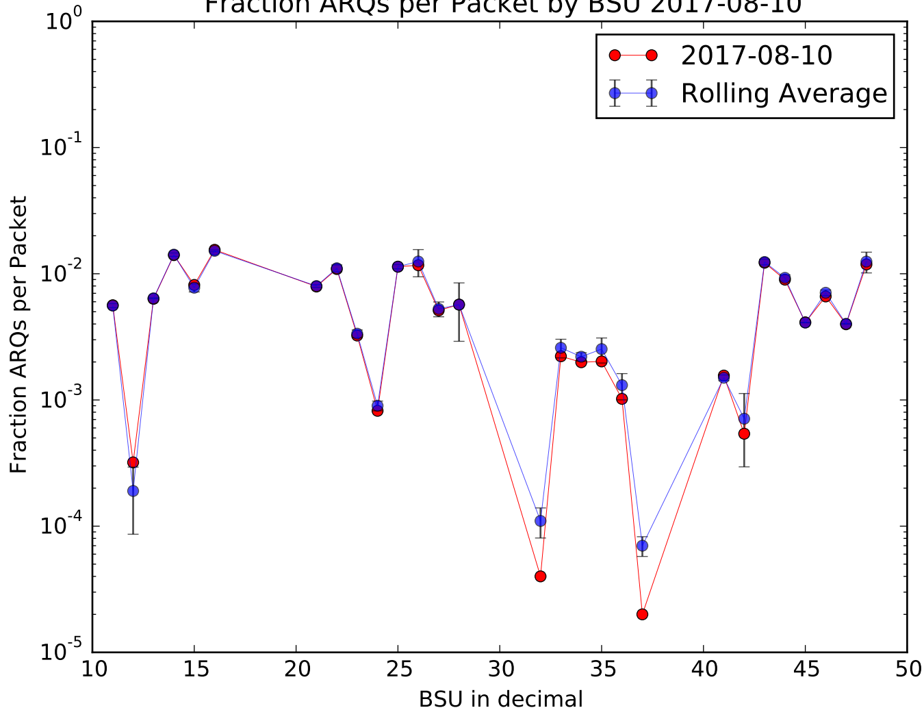
Fraction ARQs per Packet by BSU 2017-08-10
