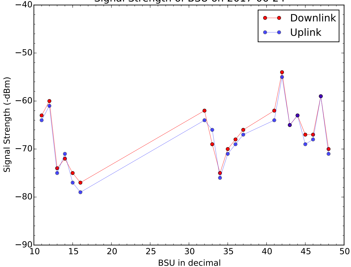
Signal Strength of BSU on 2017-06-24
