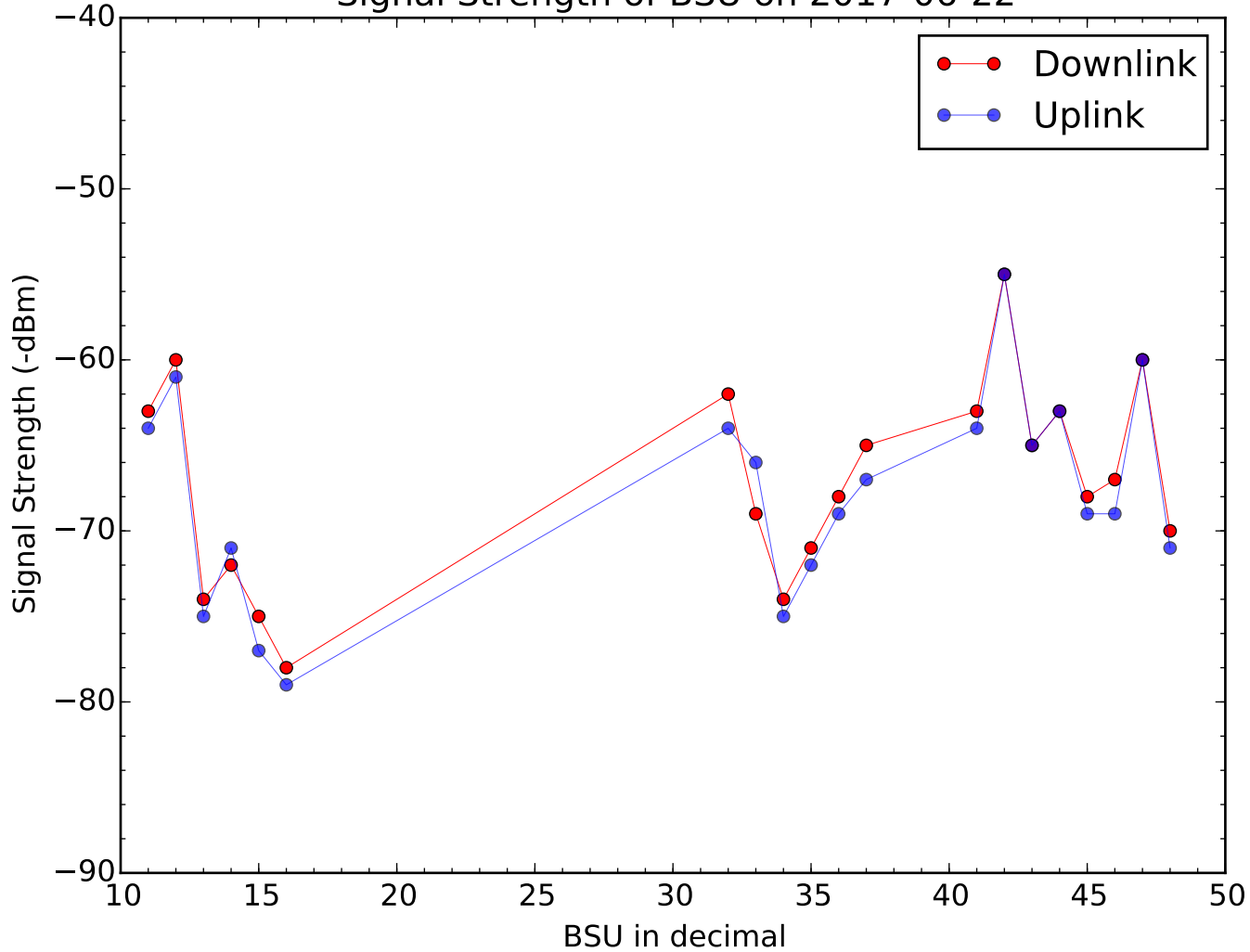
Signal Strength of BSU on 2017-06-22
