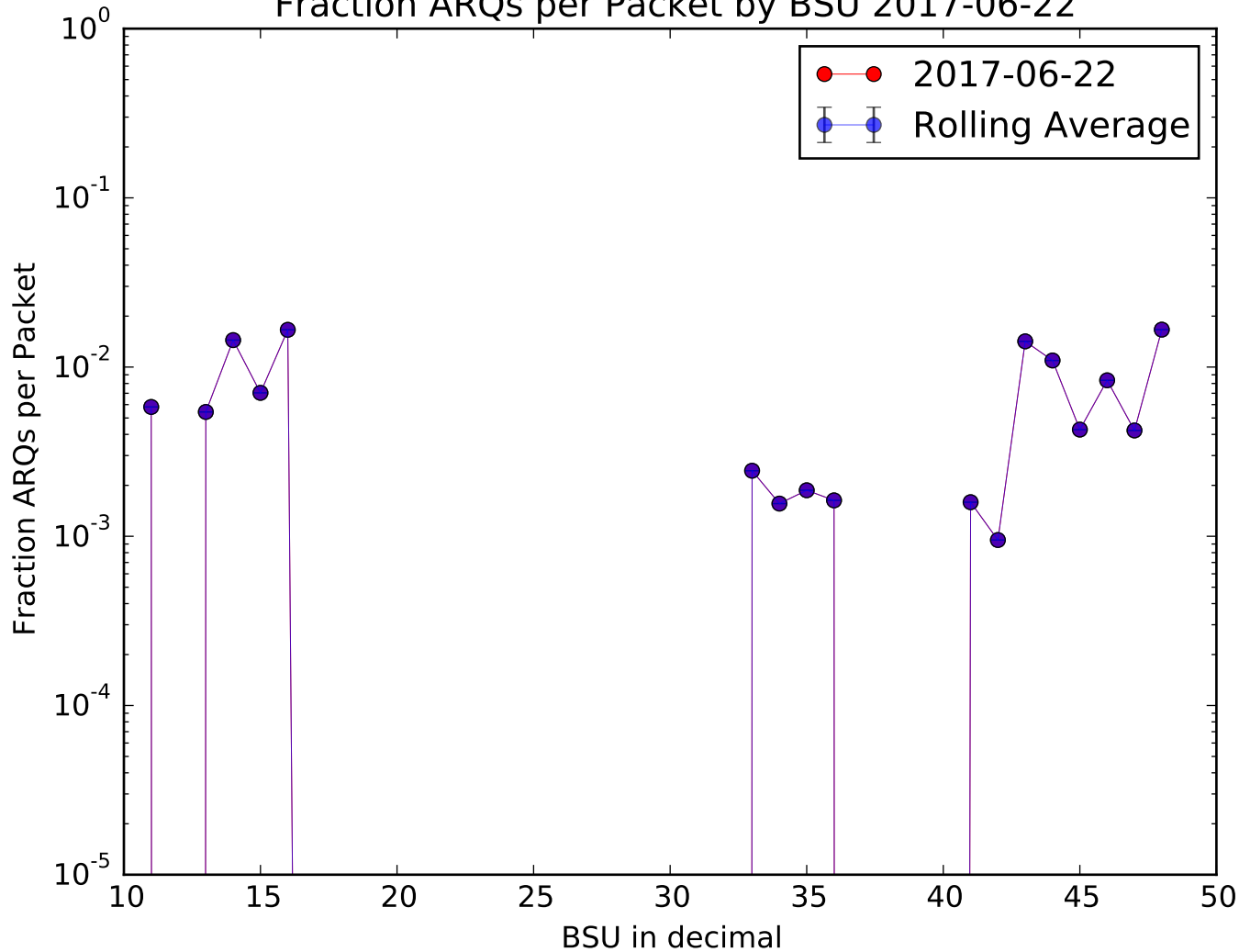
Fraction ARQs per Packet by BSU 2017-06-22
