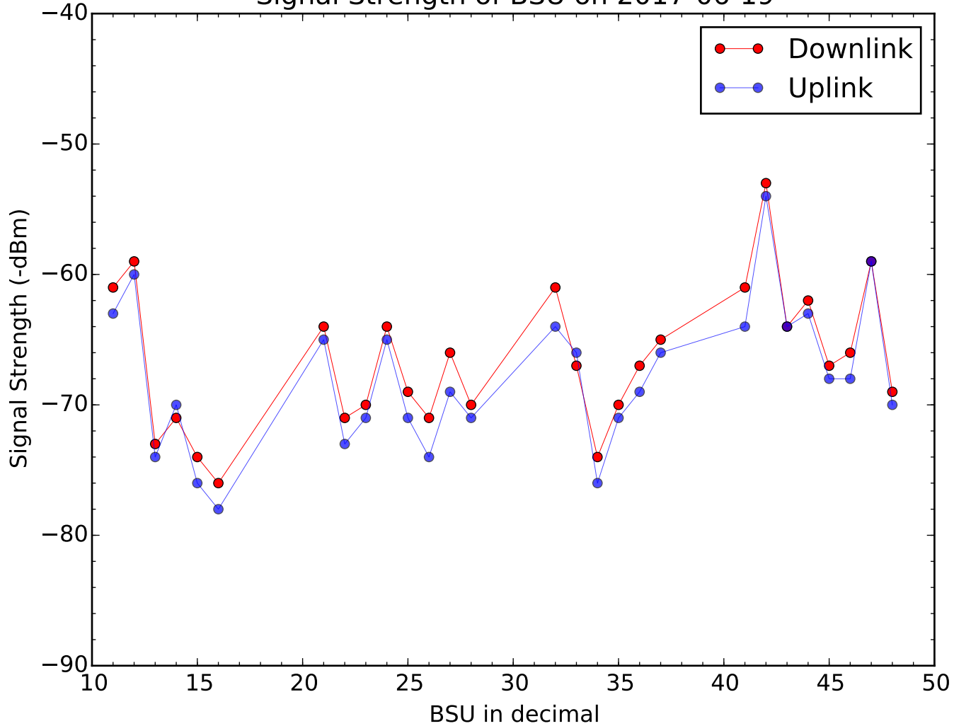
Signal Strength of BSU on 2017-06-19
