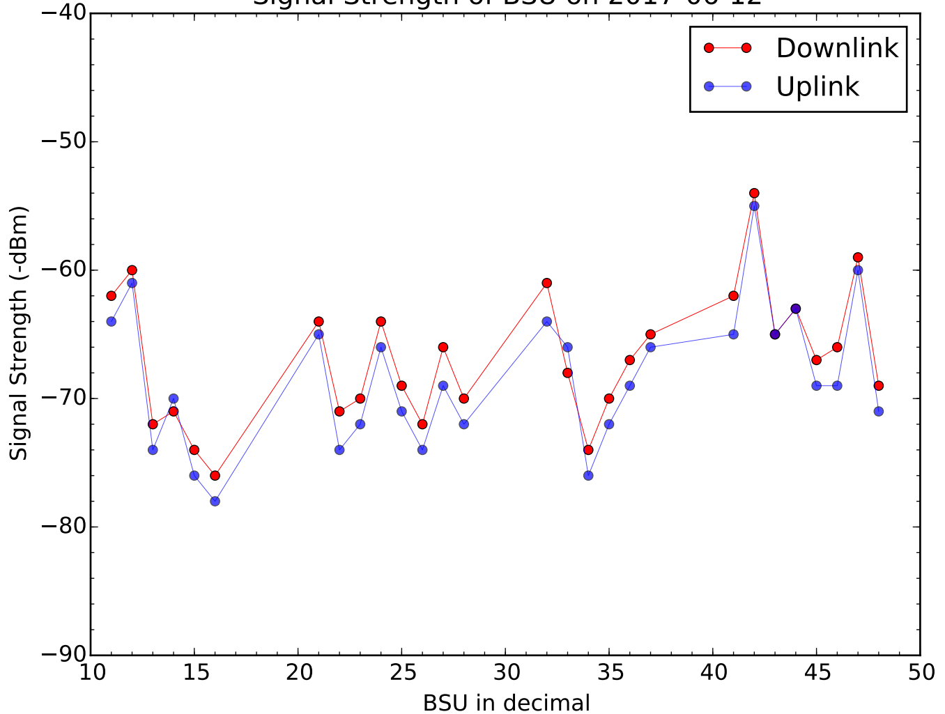
Signal Strength of BSU on 2017-06-12
