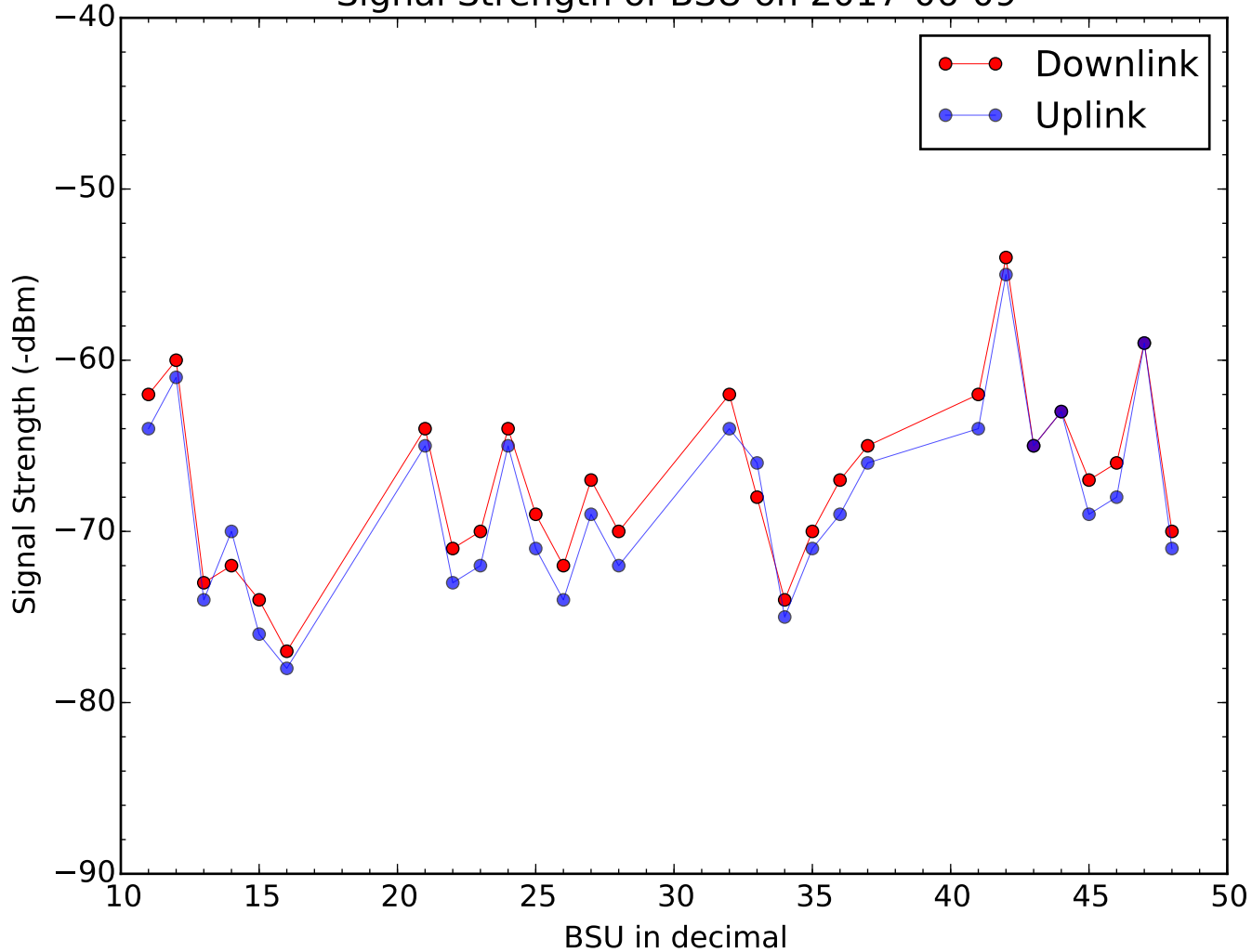
Signal Strength of BSU on 2017-06-09
