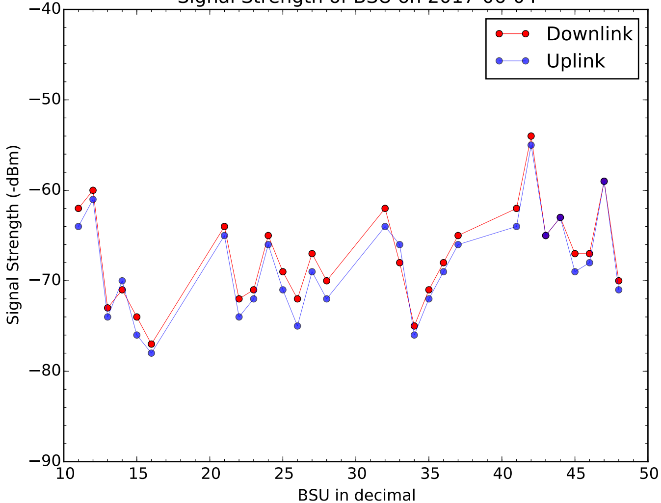
Signal Strength of BSU on 2017-06-04
