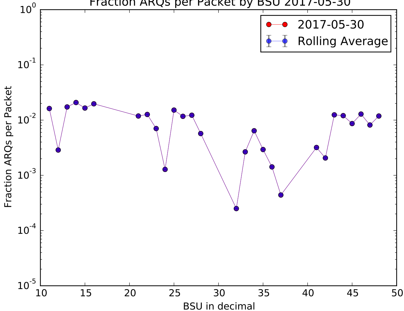
Fraction ARQs per Packet by BSU 2017-05-30
