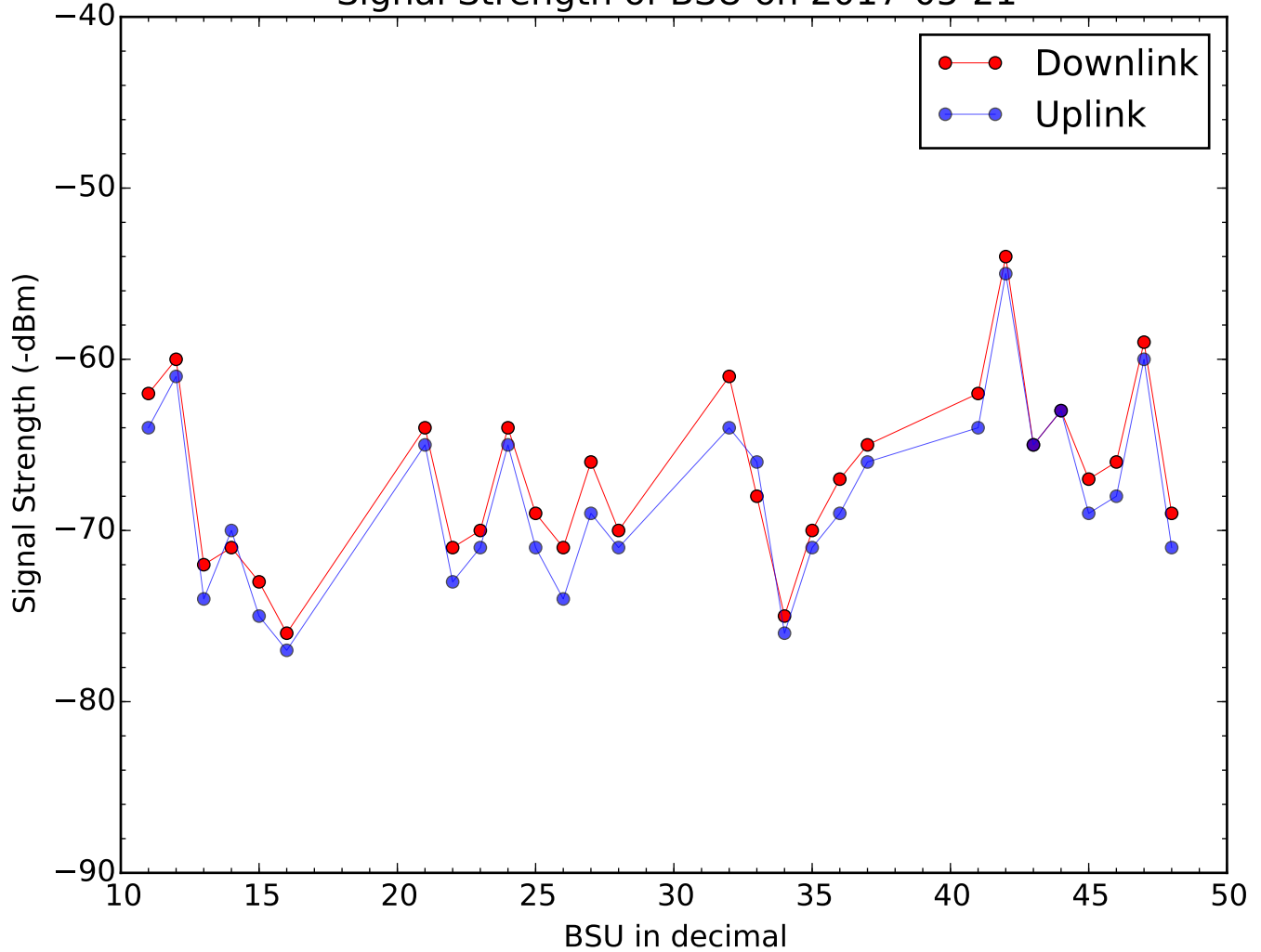
Signal Strength of BSU on 2017-05-21
