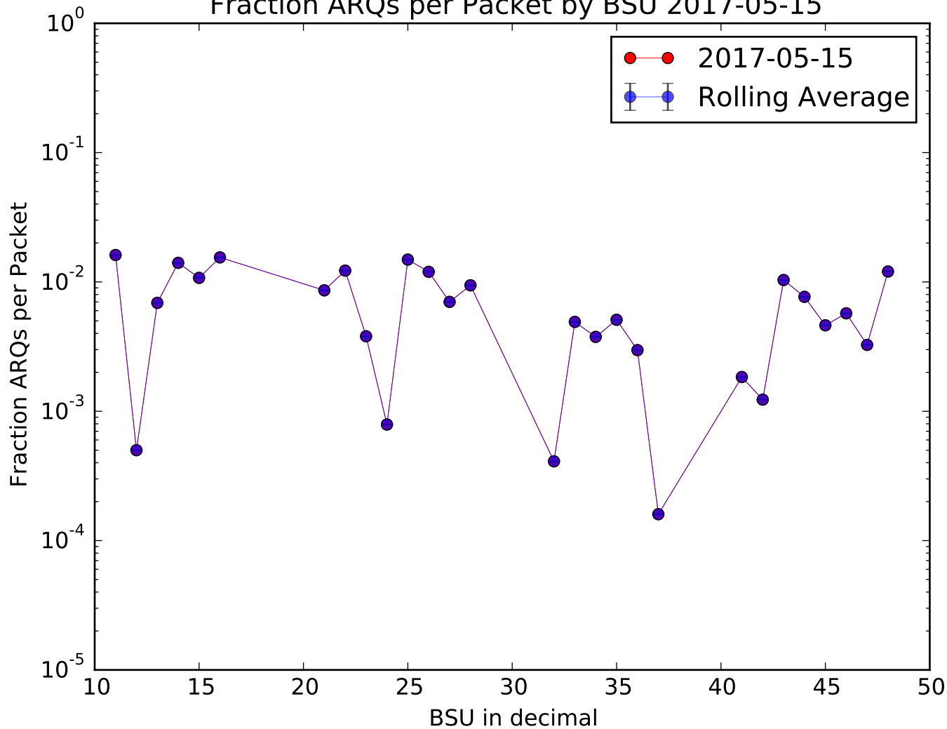
Fraction ARQs per Packet by BSU 2017-05-15
