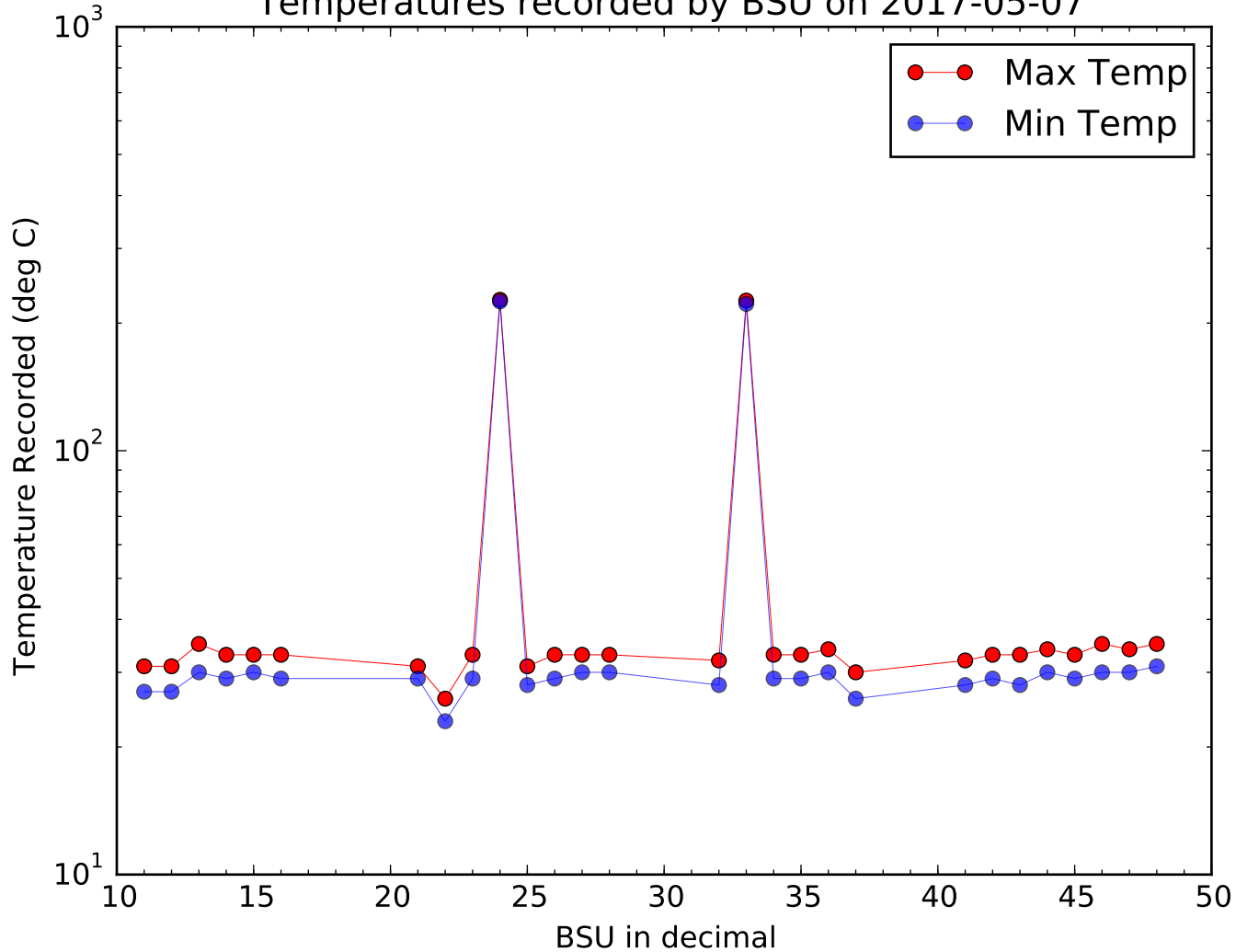
Temperatures recorded by BSU on 2017-05-07
