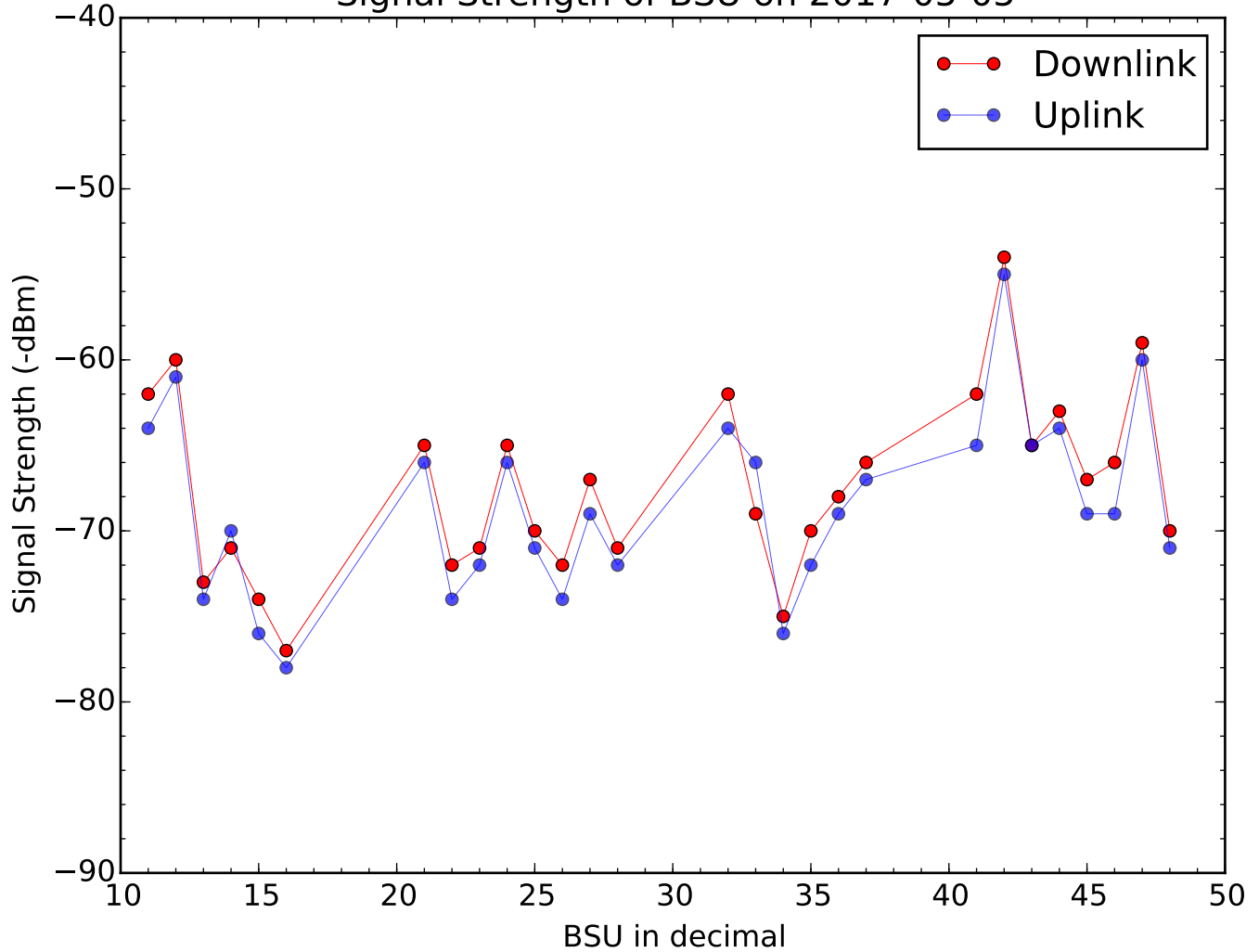
Signal Strength of BSU on 2017-05-05
