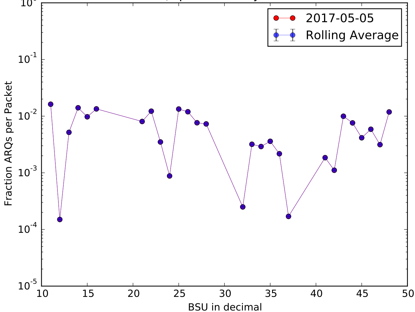
Fraction ARQs per Packet by BSU 2017-05-05
