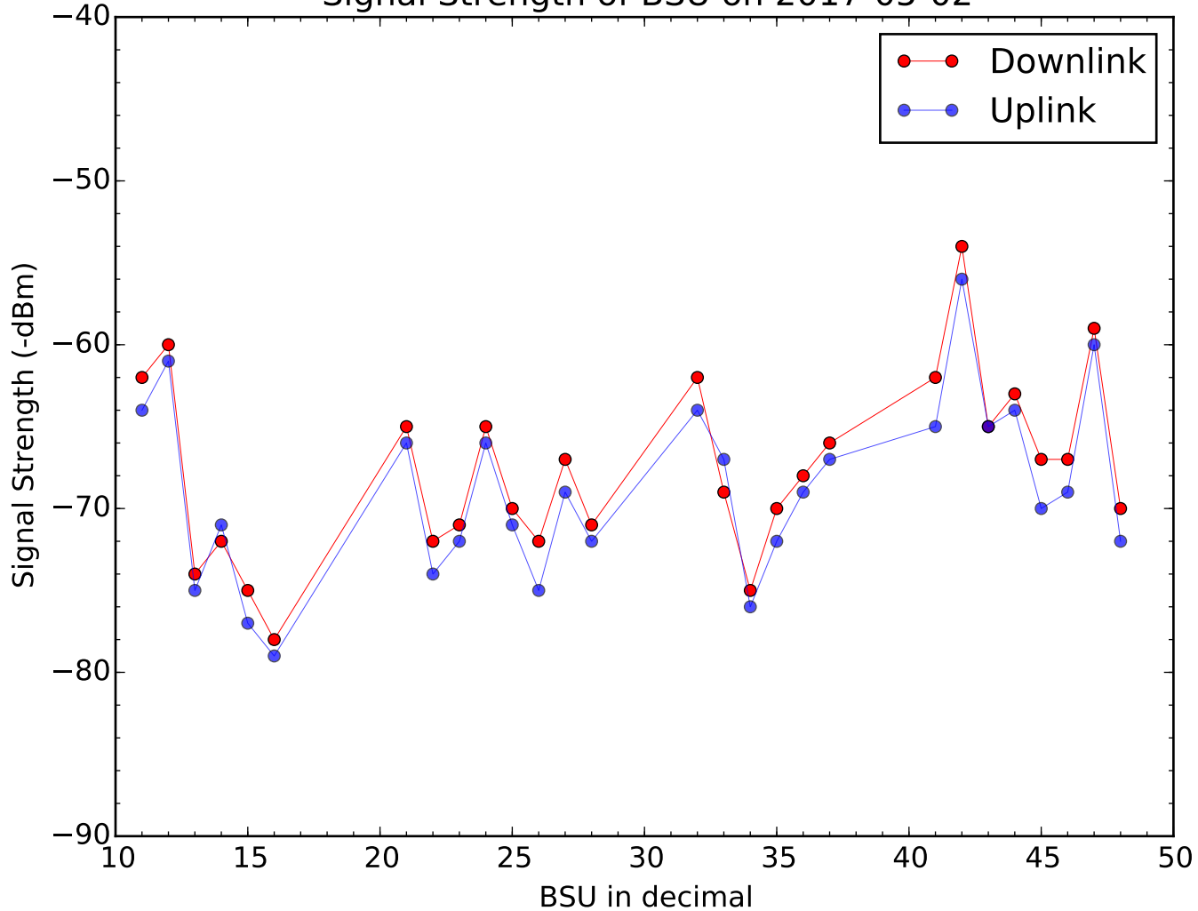
Signal Strength of BSU on 2017-05-02
