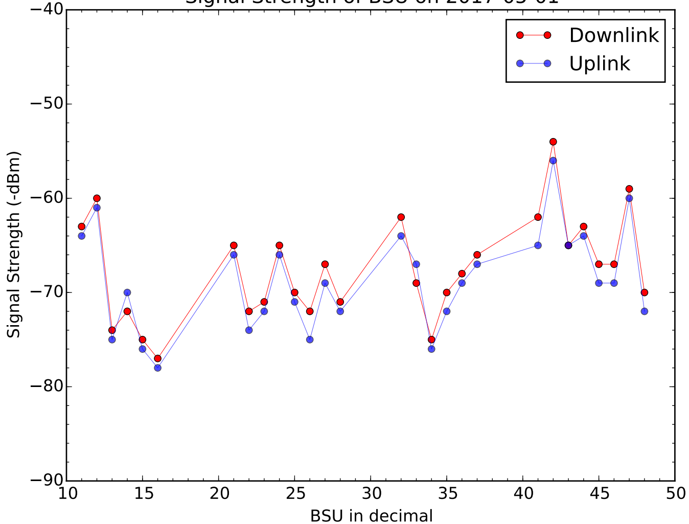
Signal Strength of BSU on 2017-05-01
