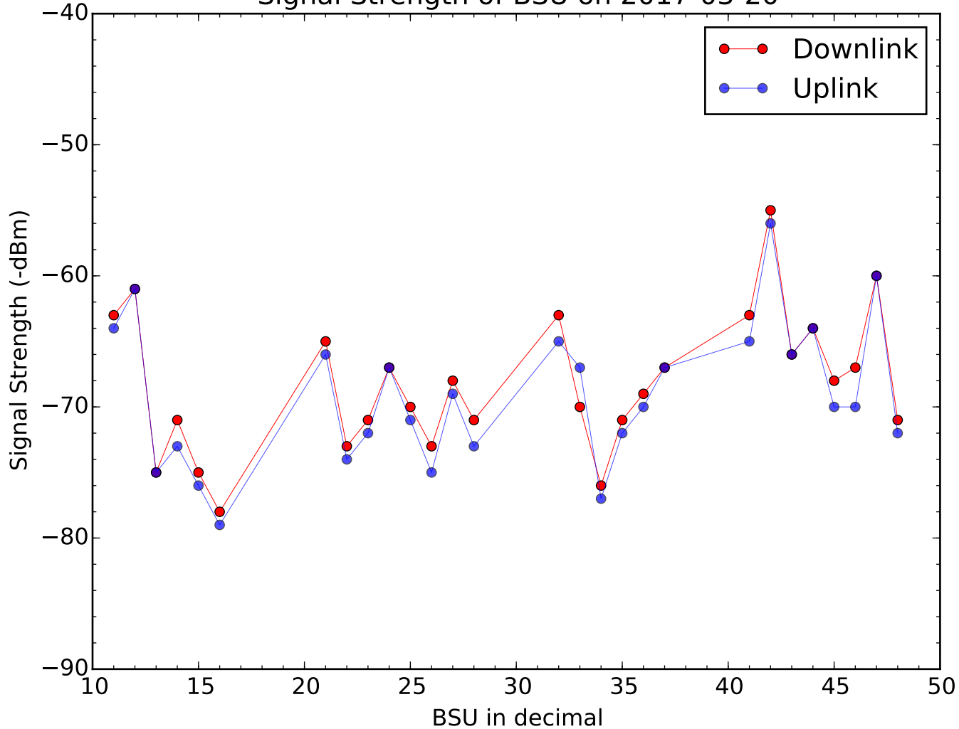
Signal Strength of BSU on 2017-03-20
