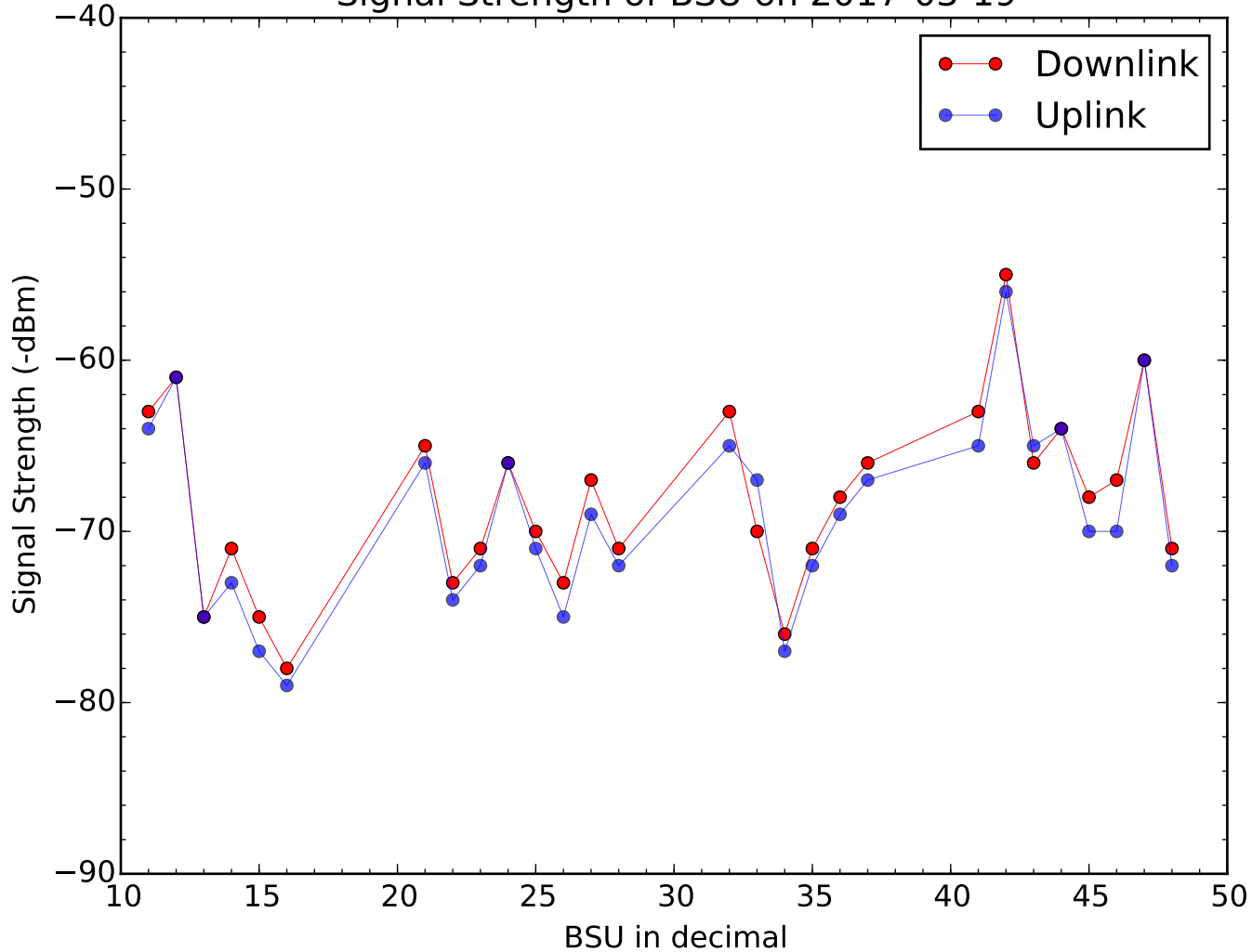
Signal Strength of BSU on 2017-03-19
