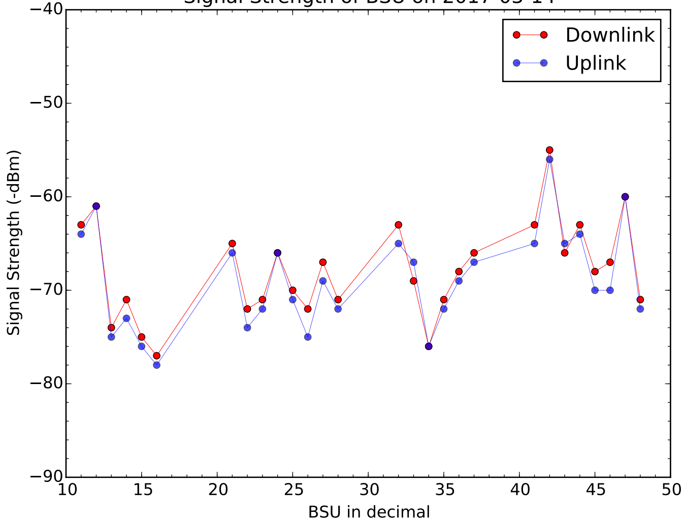
Signal Strength of BSU on 2017-03-14
