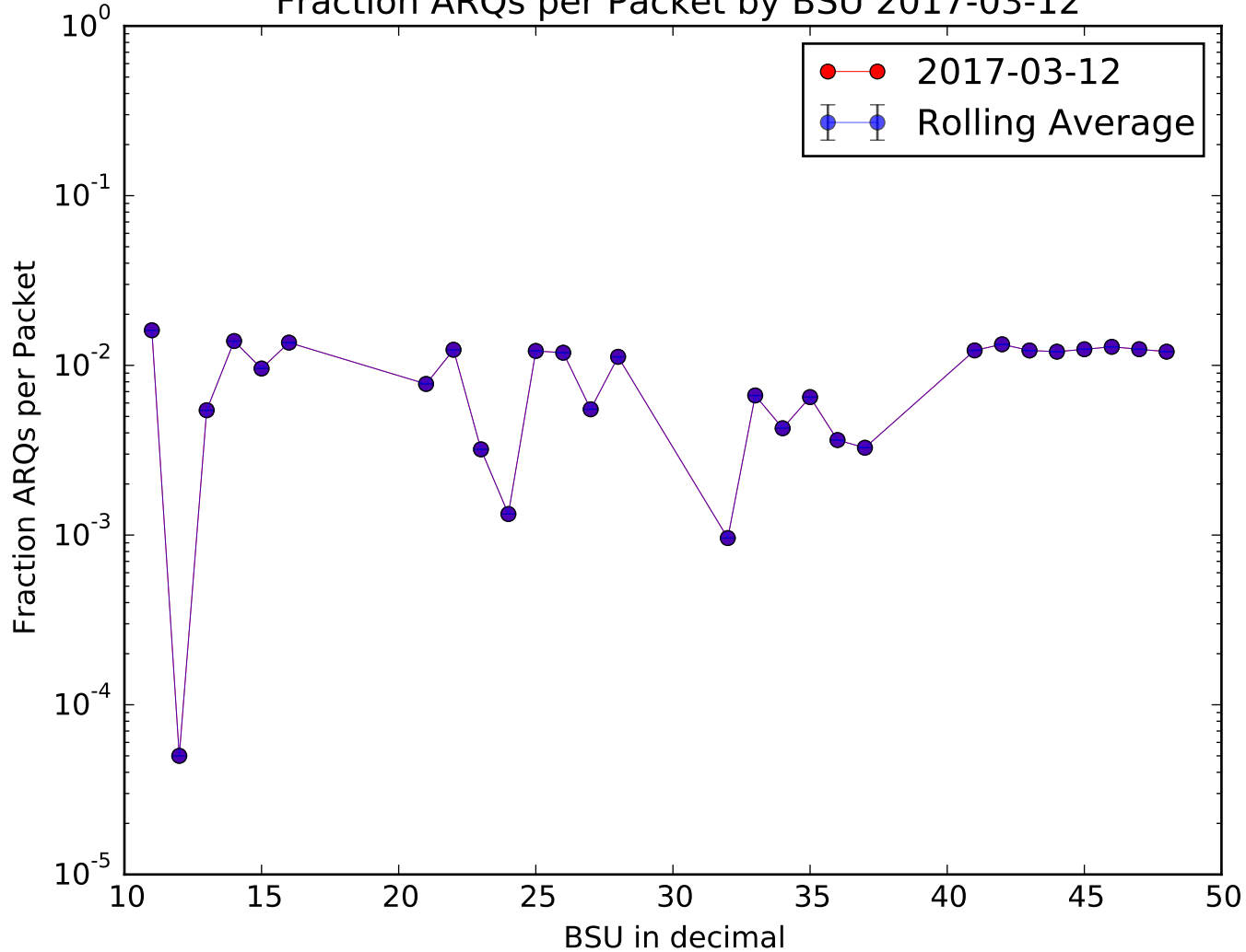
Fraction ARQs per Packet by BSU 2017-03-12
