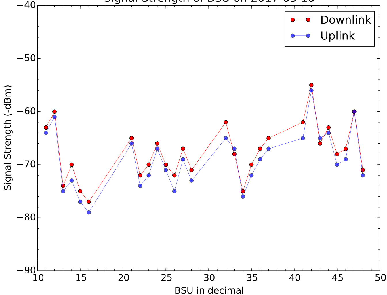
Signal Strength of BSU on 2017-03-10
