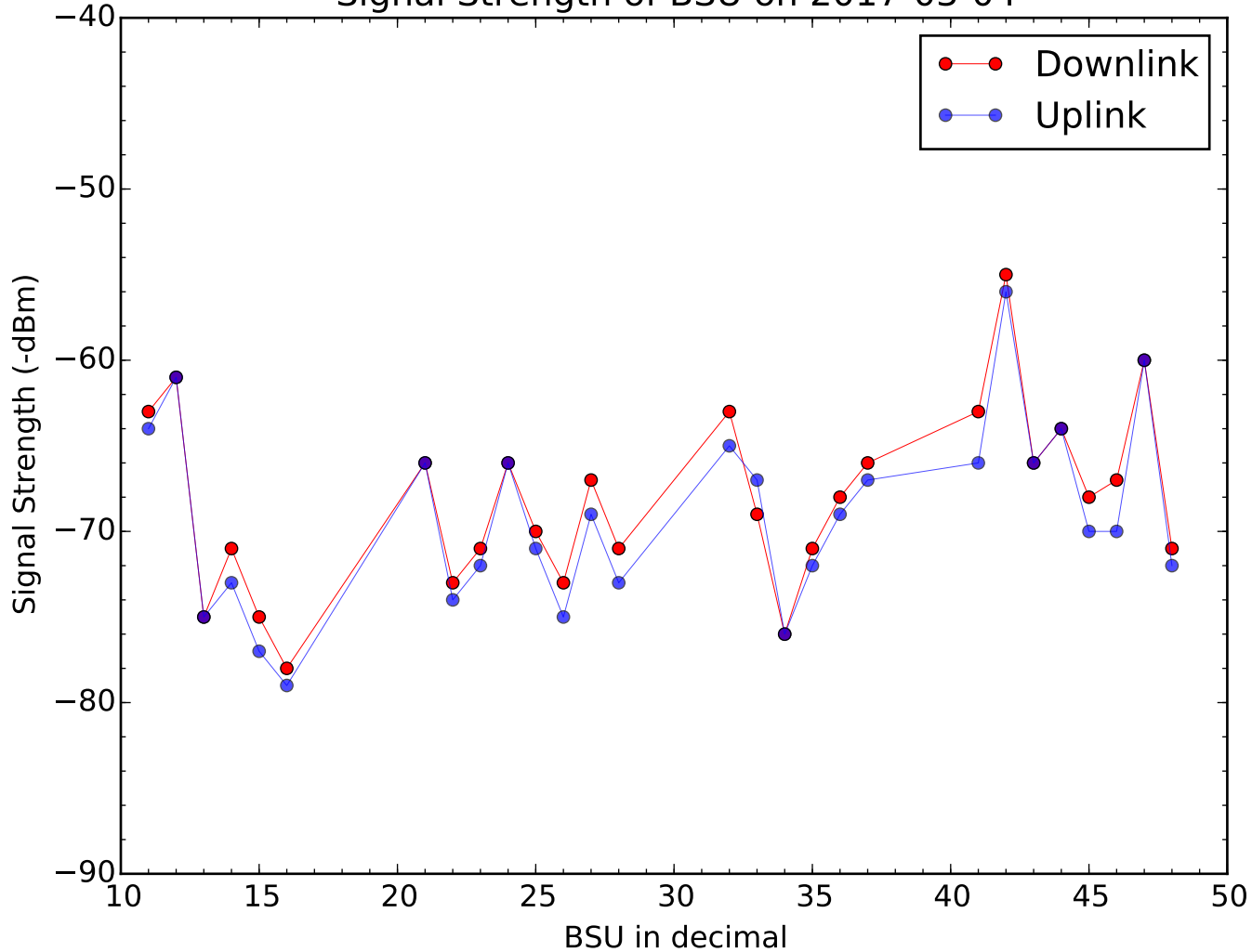
Signal Strength of BSU on 2017-03-04
