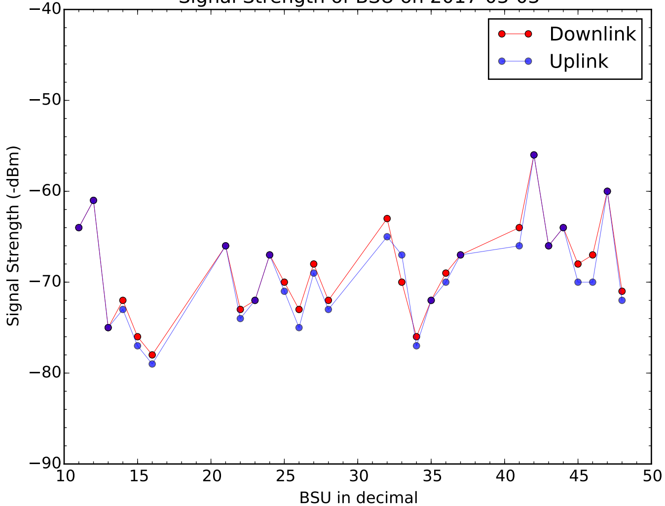
Signal Strength of BSU on 2017-03-03
