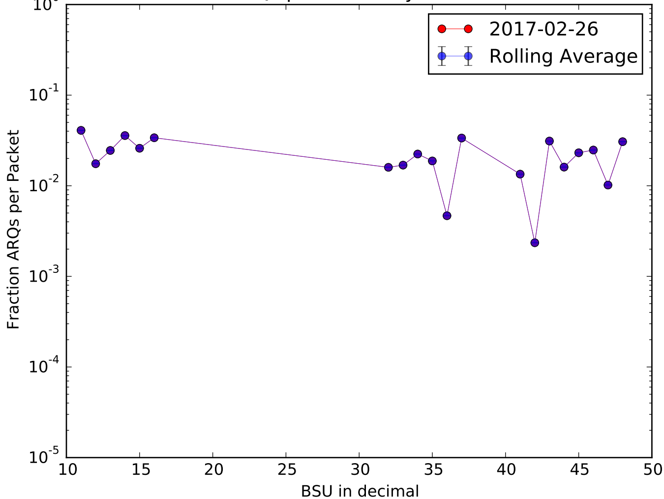
Fraction ARQs per Packet by BSU 2017-02-26
