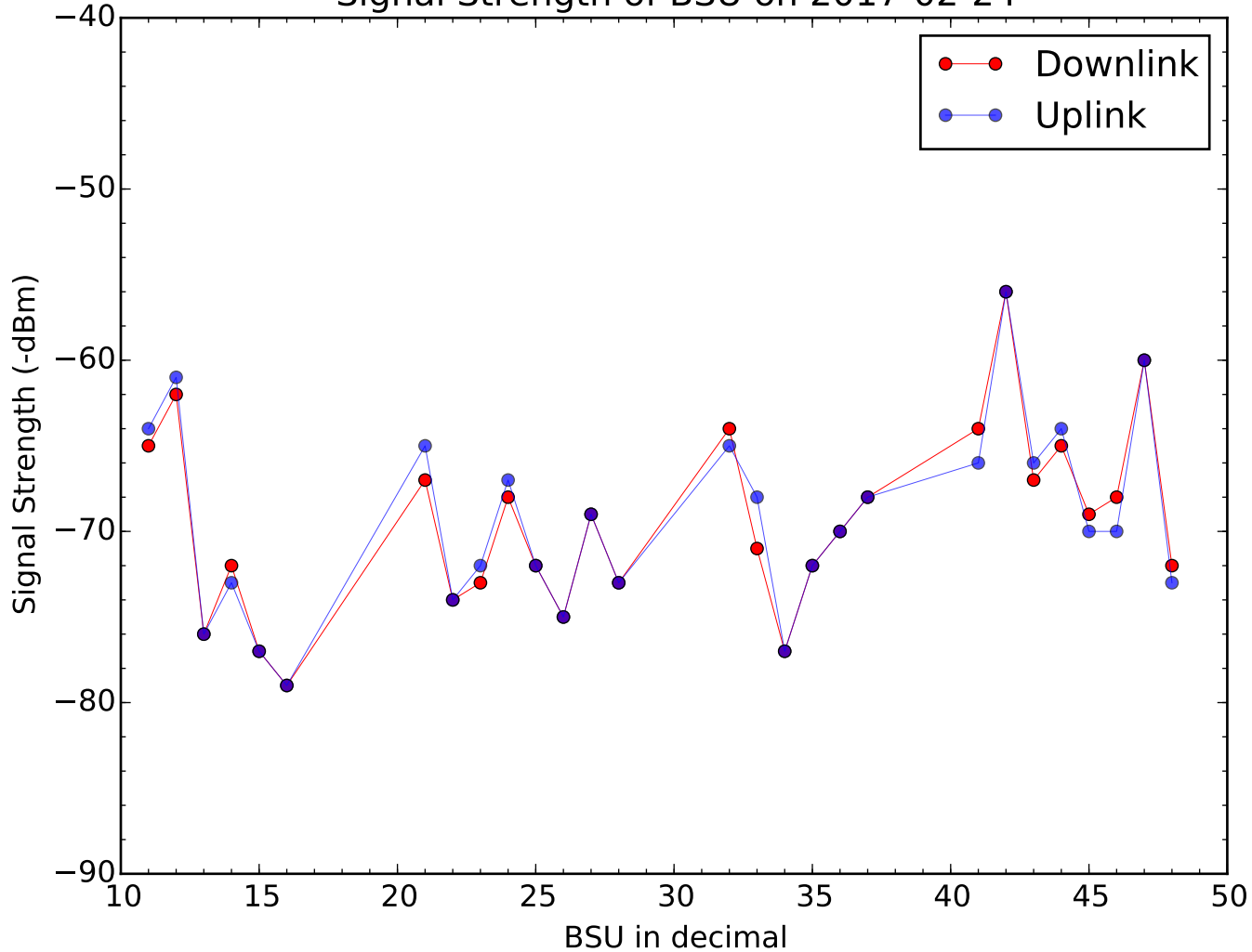
Signal Strength of BSU on 2017-02-24
