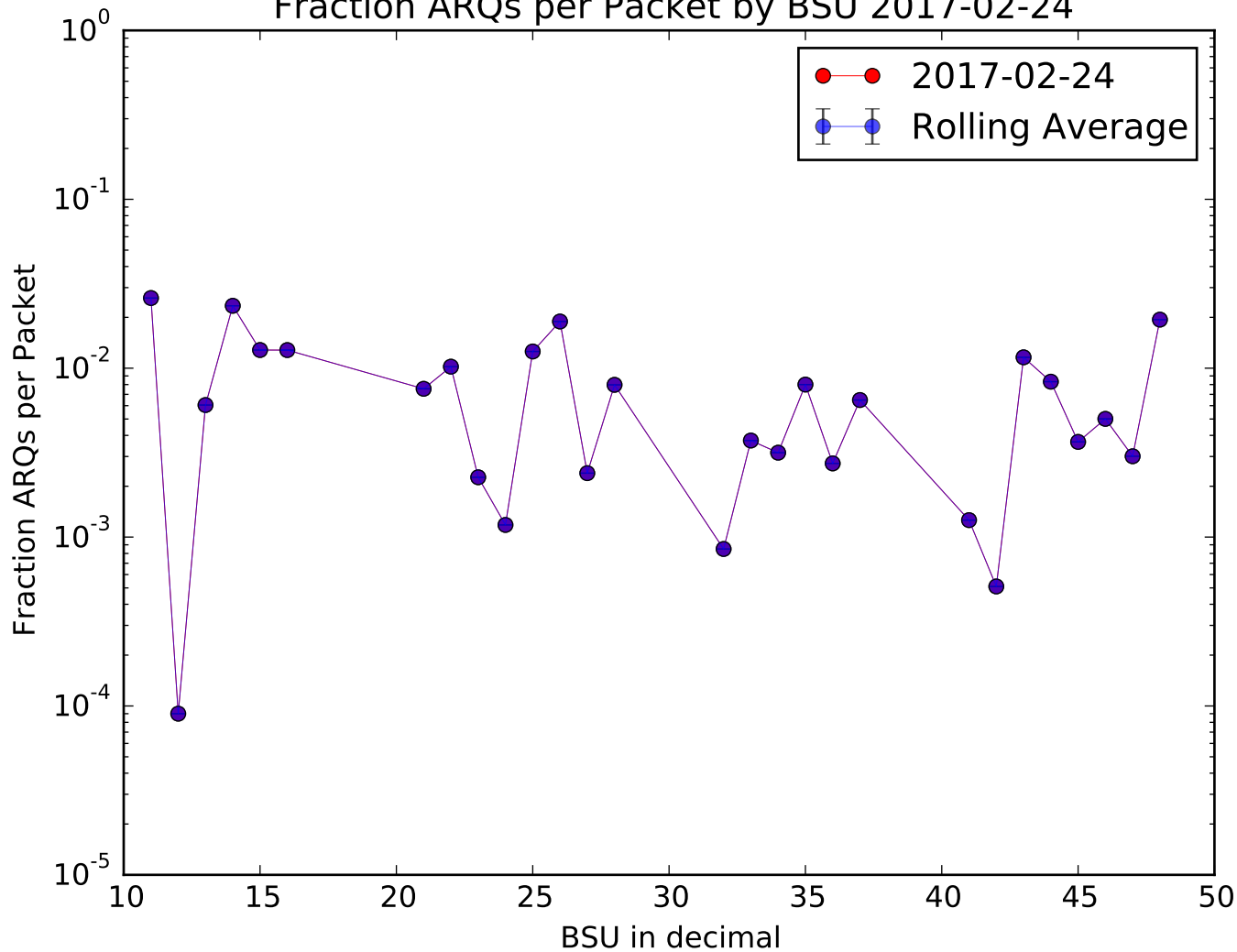
Fraction ARQs per Packet by BSU 2017-02-24
