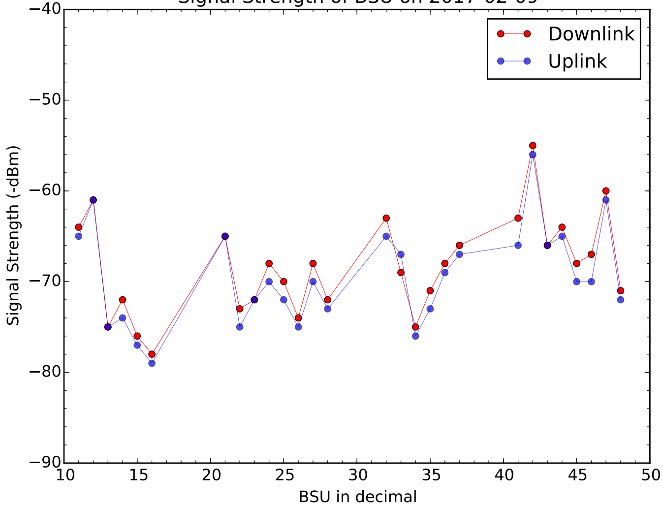
Signal Strength of BSU on 2017-02-09
