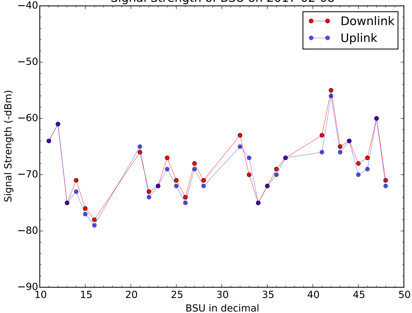
Signal Strength of BSU on 2017-02-08
