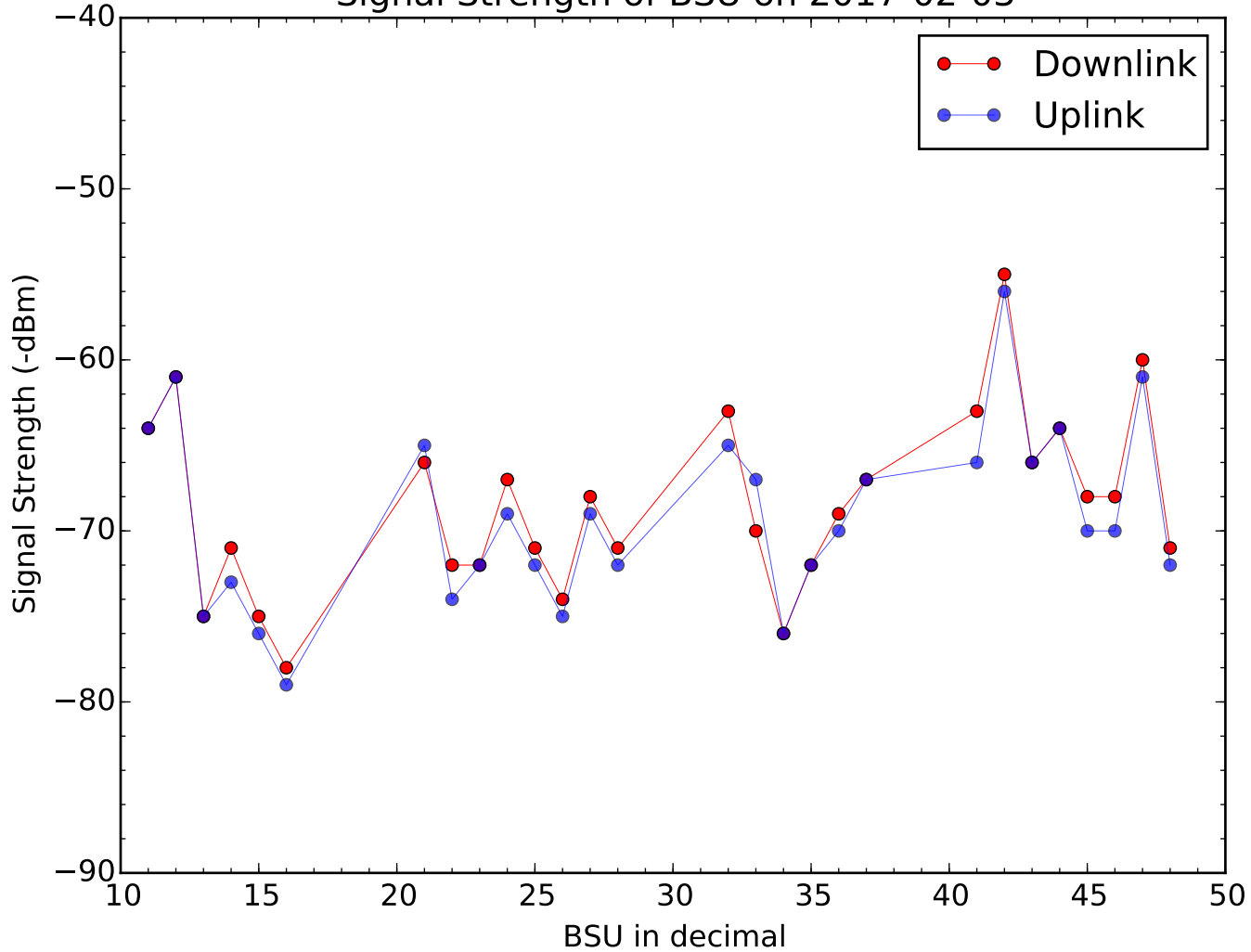
Signal Strength of BSU on 2017-02-03
