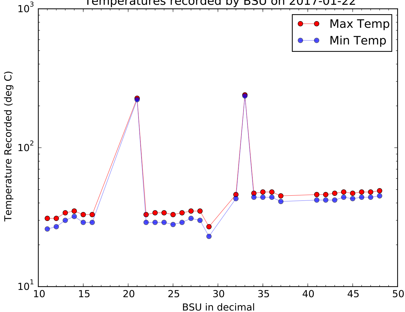
Temperatures recorded by BSU on 2017-01-22
