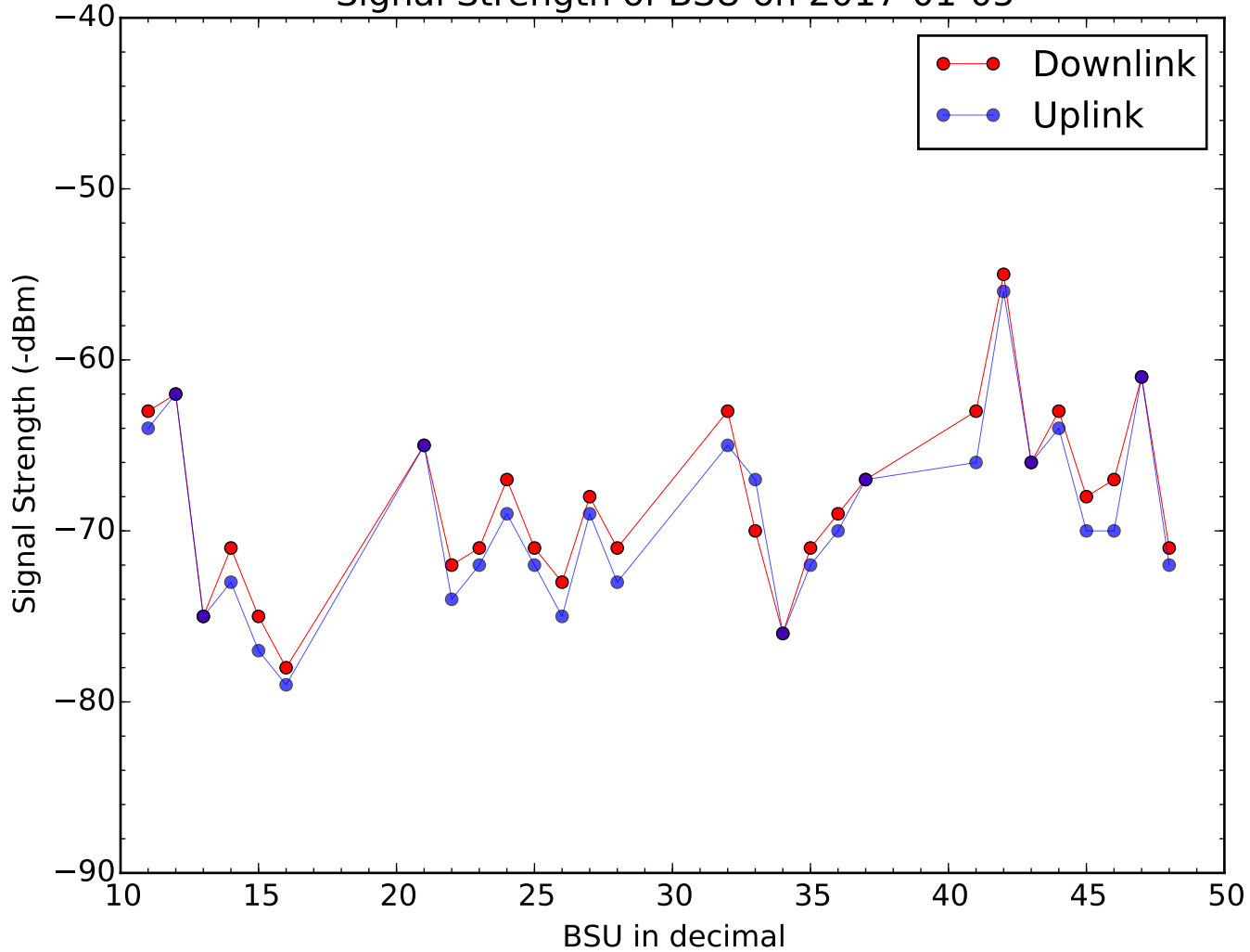
Signal Strength of BSU on 2017-01-05
