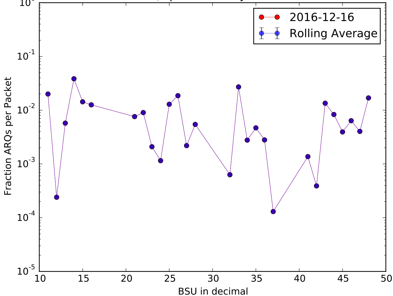
Fraction ARQs per Packet by BSU 2016-12-16
