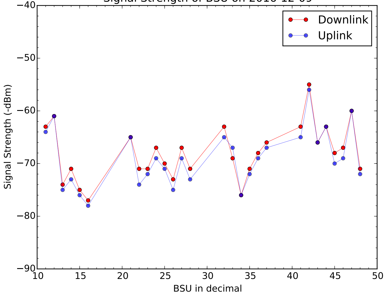
Signal Strength of BSU on 2016-12-09
