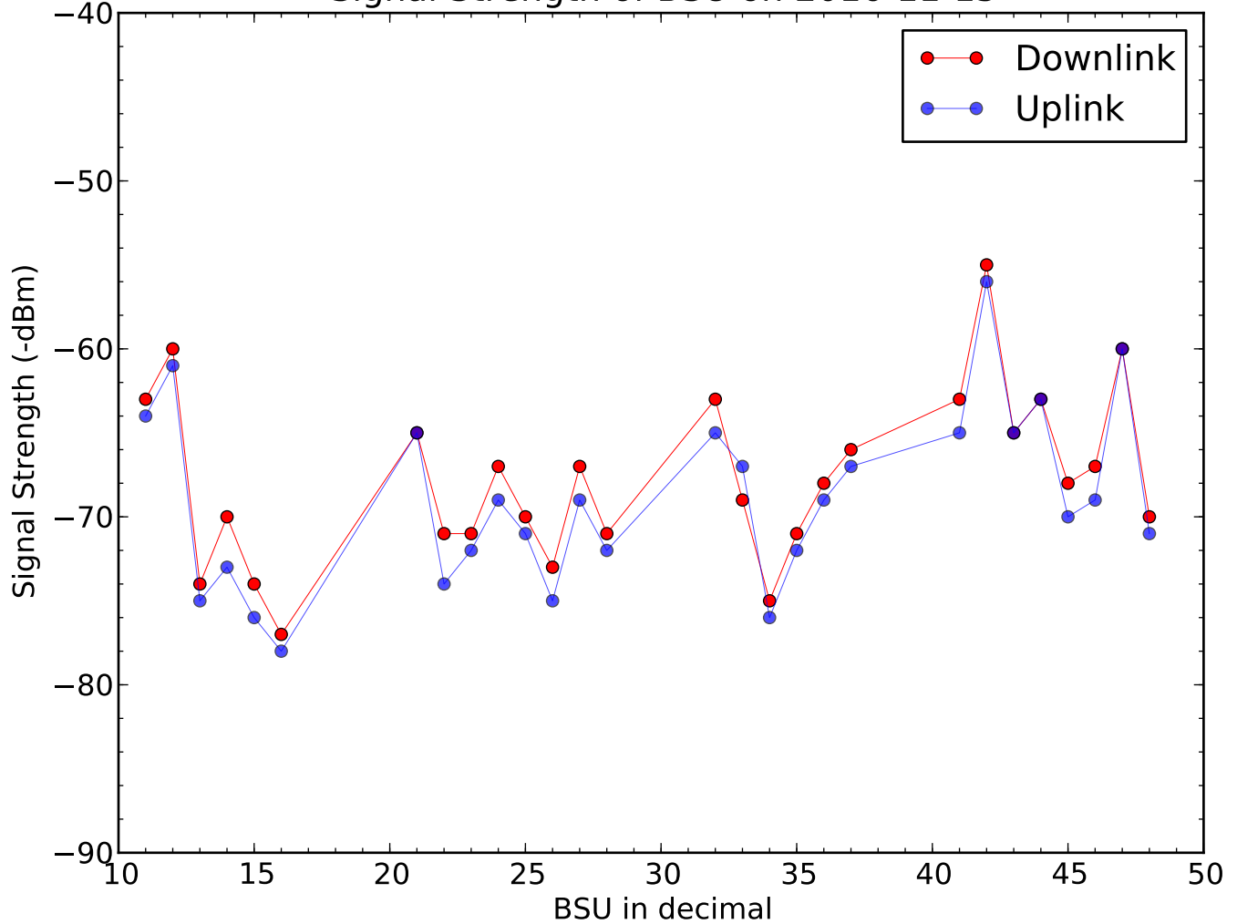
Signal Strength of BSU on 2016-11-15
