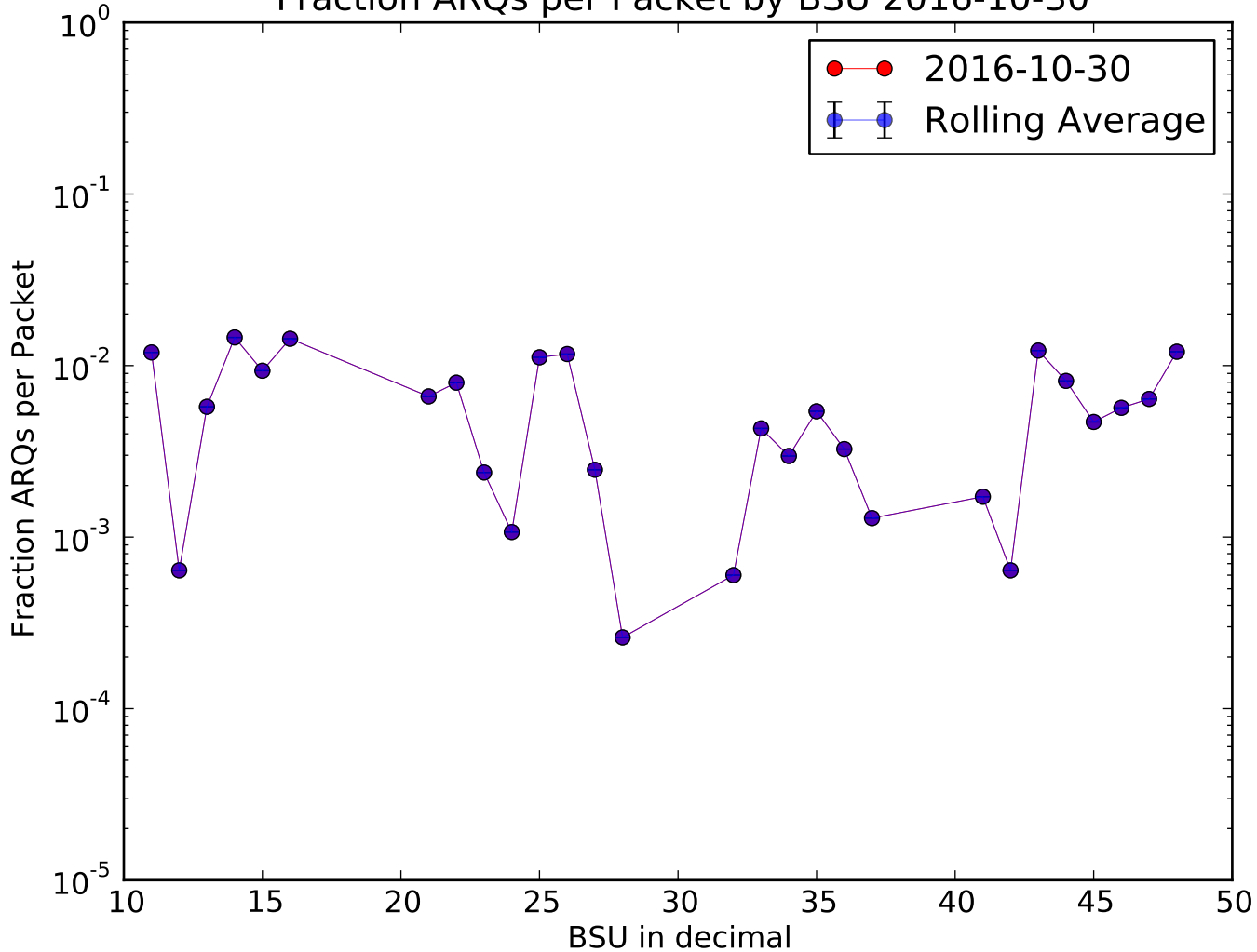
Fraction ARQs per Packet by BSU 2016-10-30
