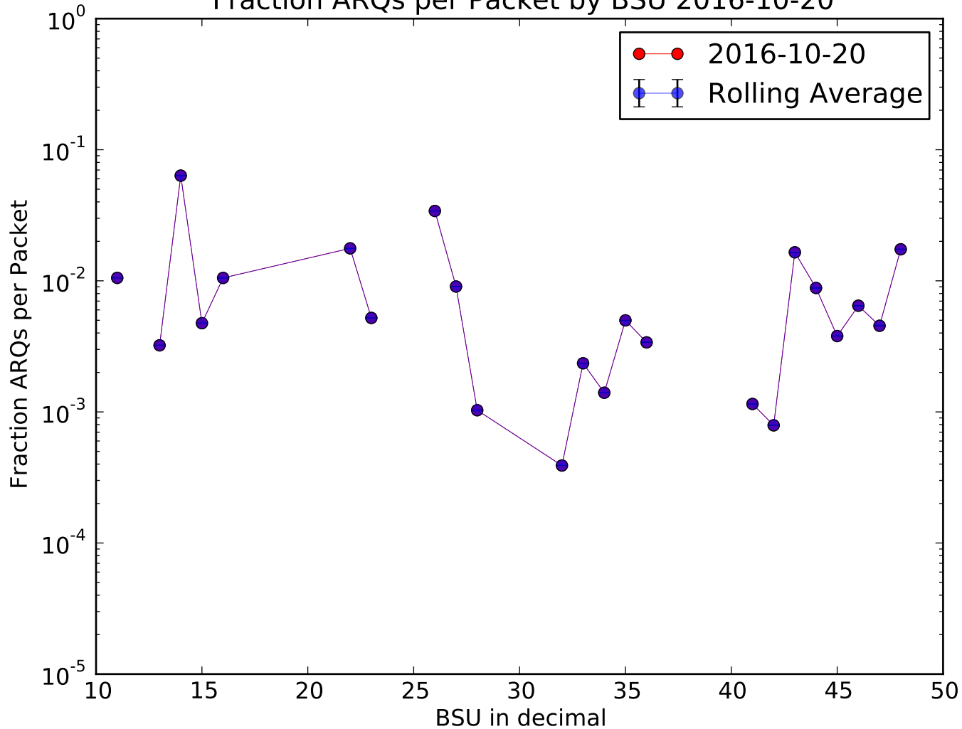
Fraction ARQs per Packet by BSU 2016-10-20
