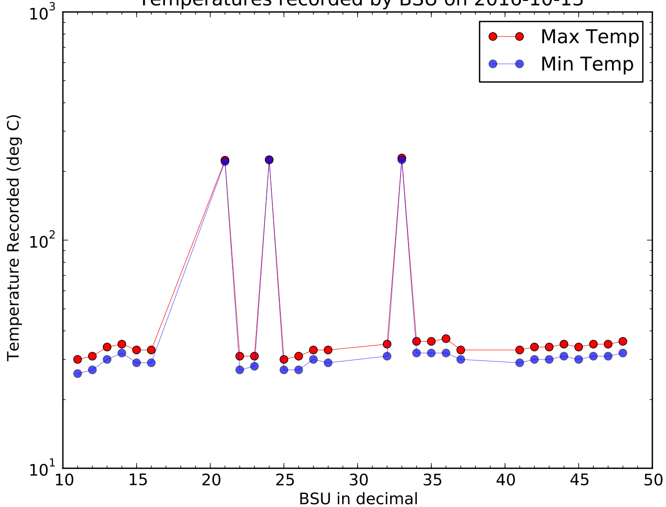
Temperatures recorded by BSU on 2016-10-13
