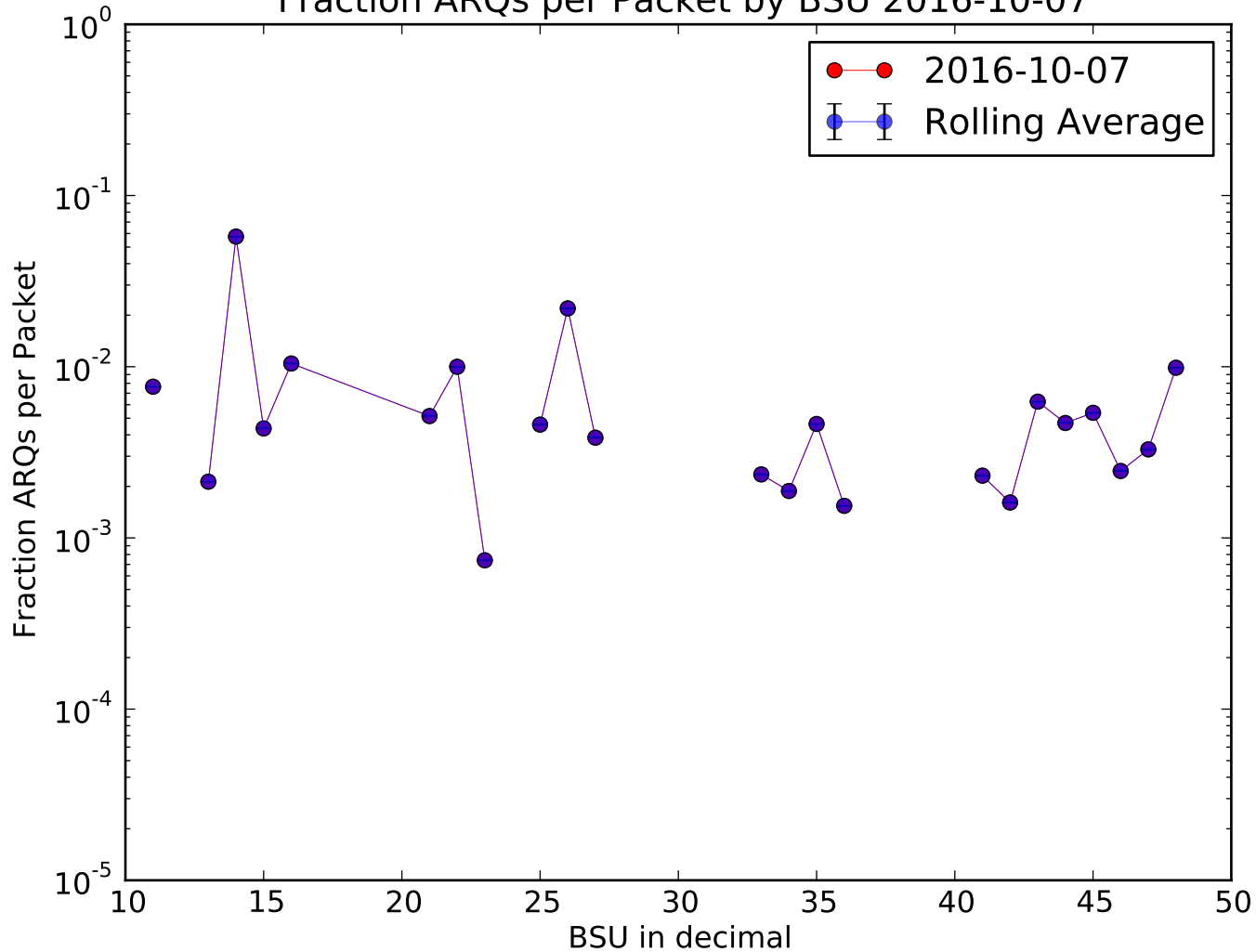
Fraction ARQs per Packet by BSU 2016-10-07
