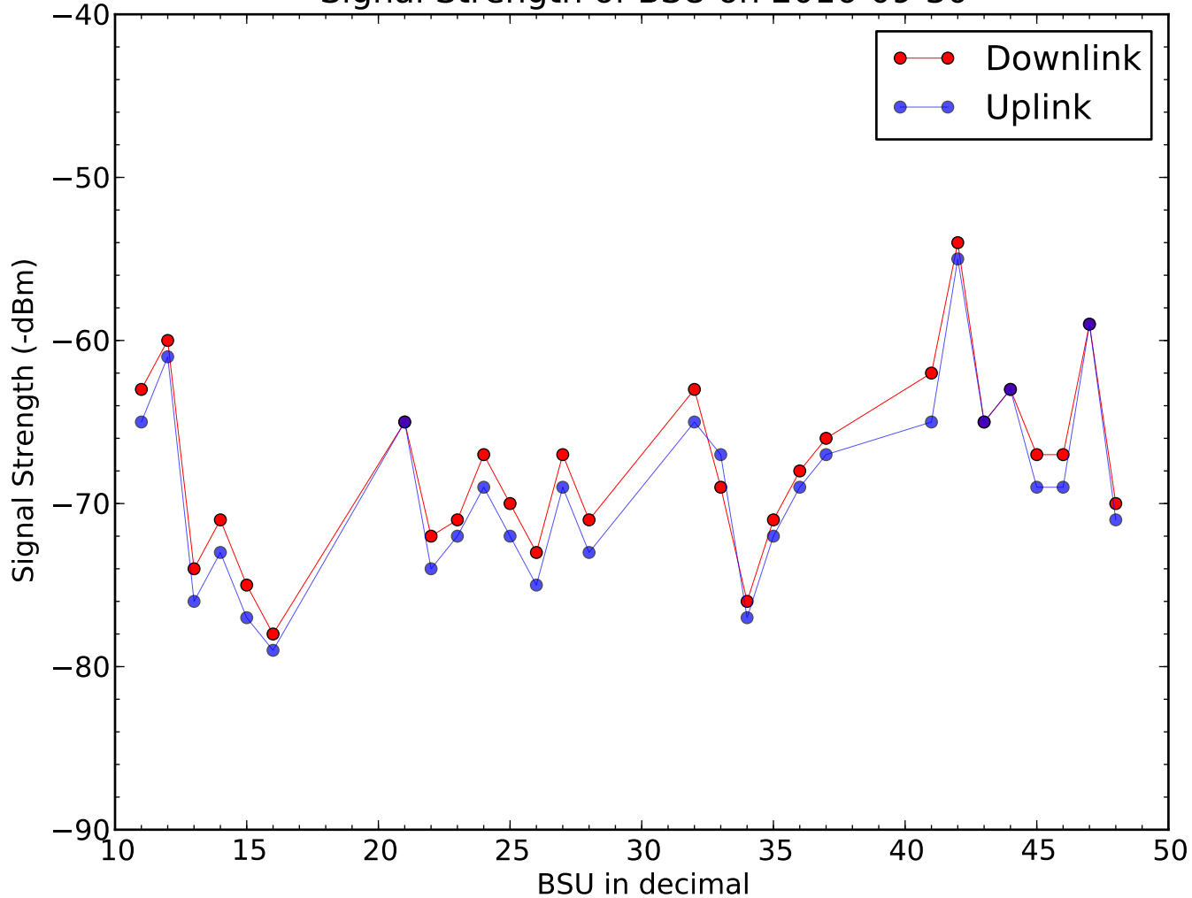
Signal Strength of BSU on 2016-09-30
