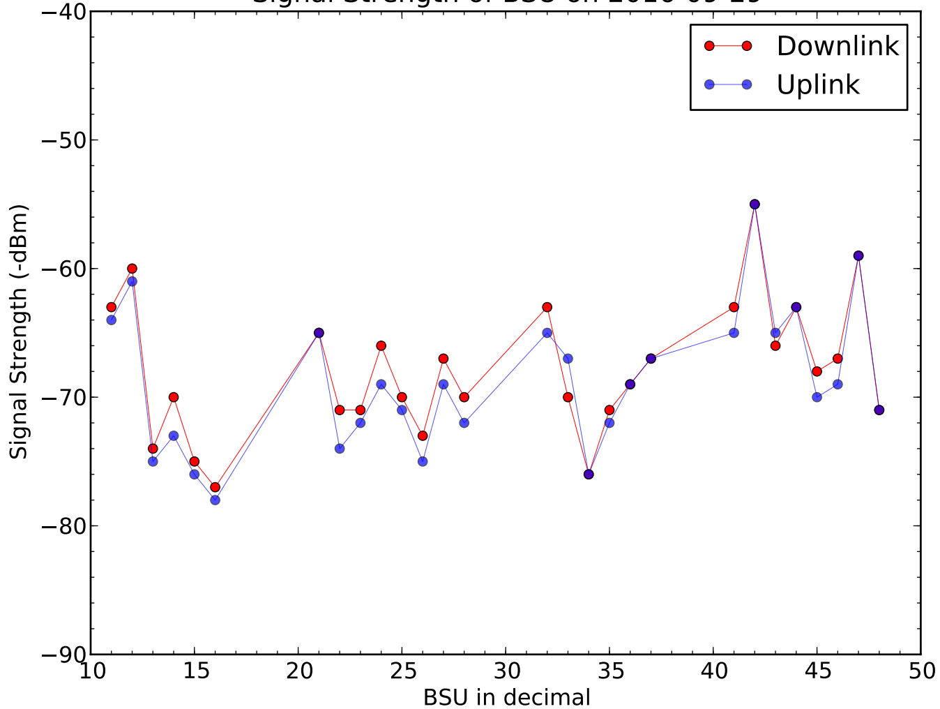
Signal Strength of BSU on 2016-09-29
