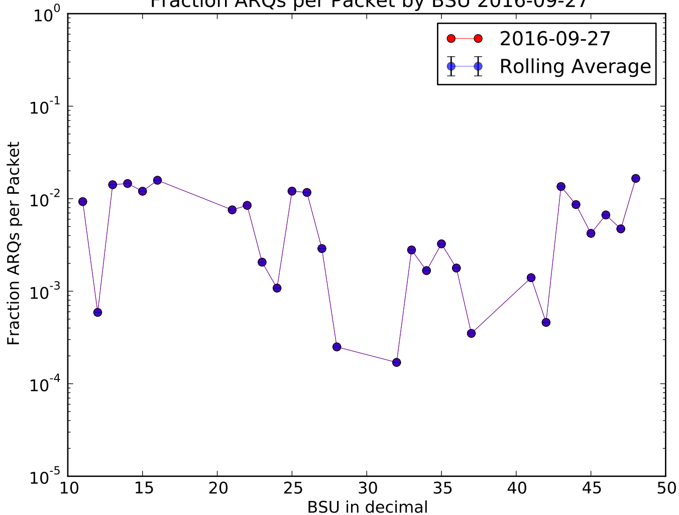
Fraction ARQs per Packet by BSU 2016-09-27
