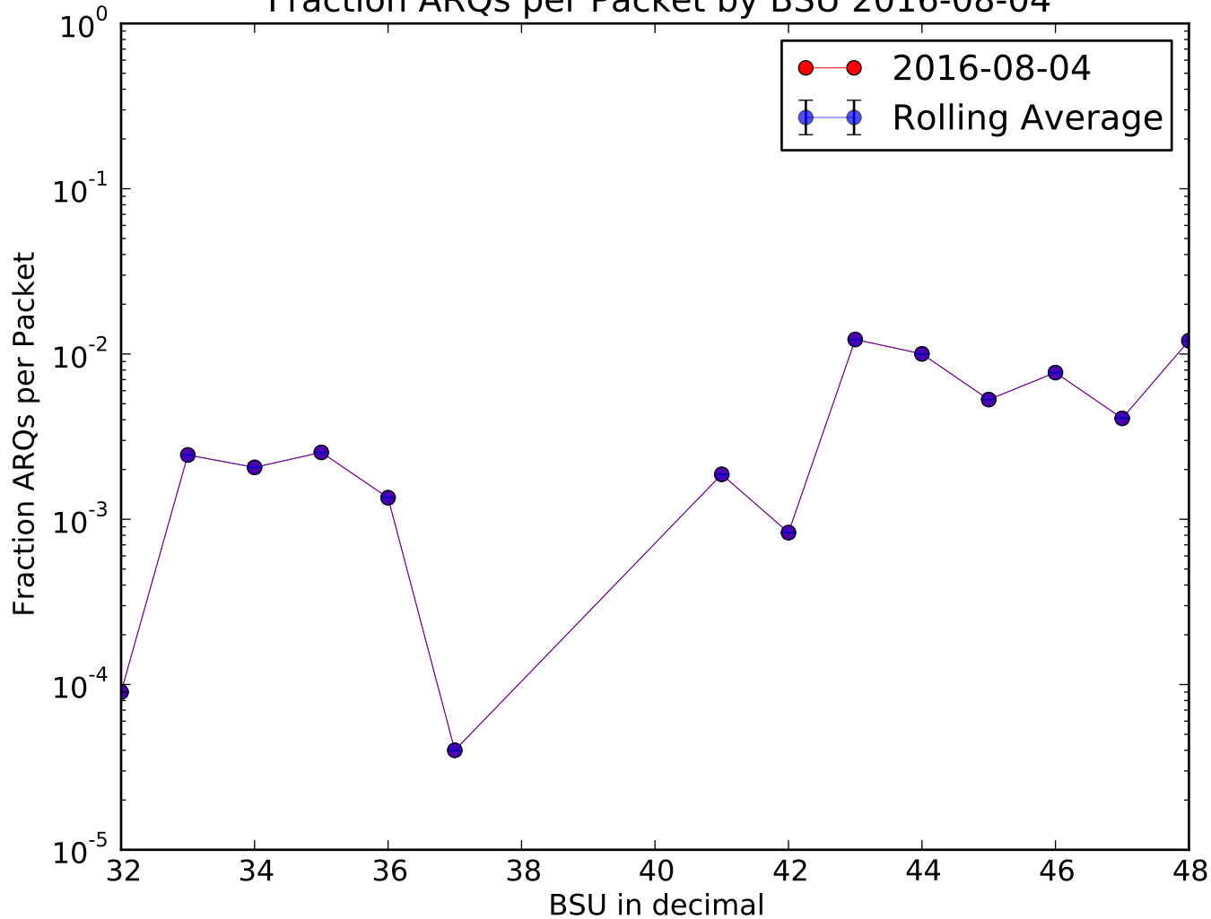
Fraction ARQs per Packet by BSU 2016-08-04
