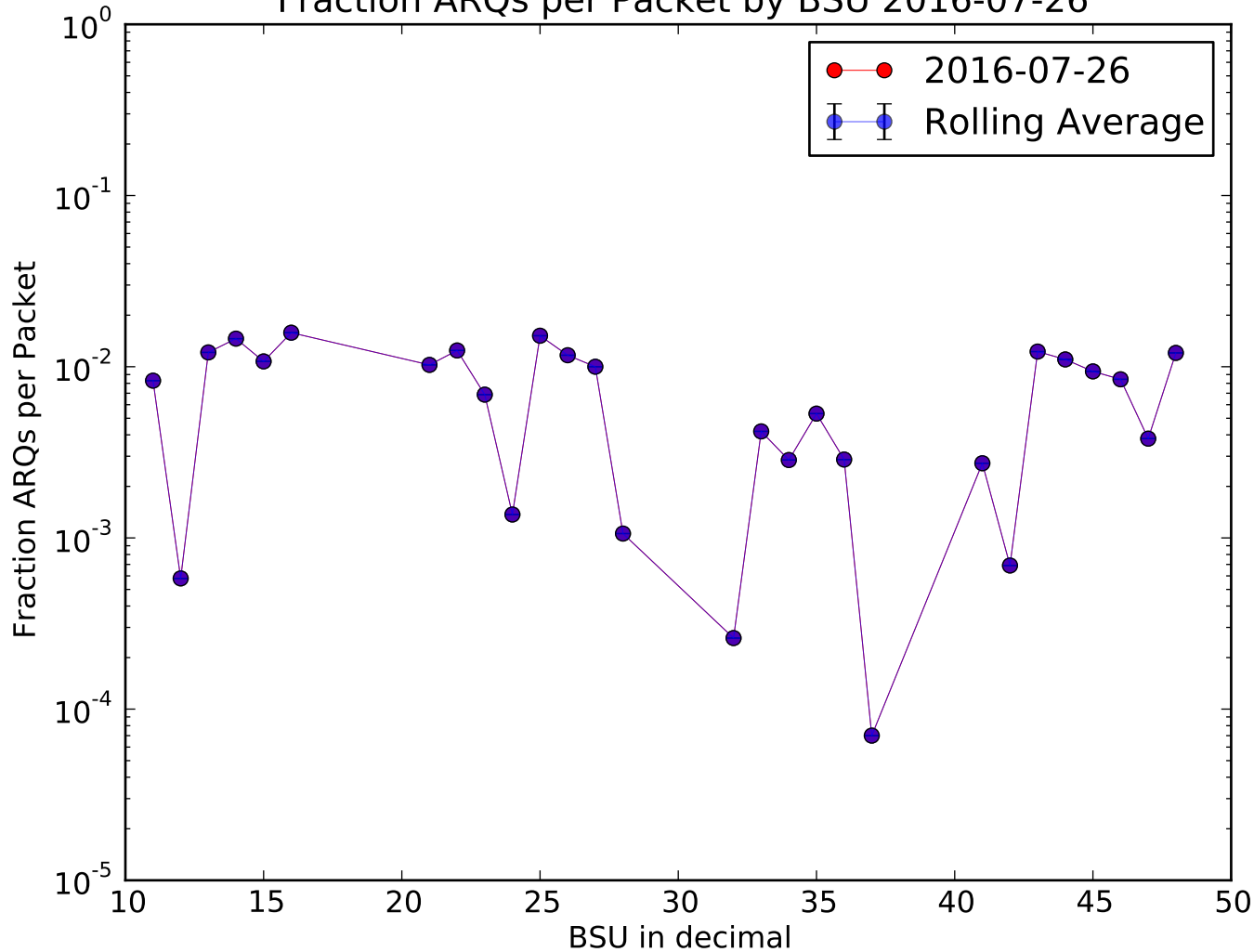
Fraction ARQs per Packet by BSU 2016-07-26
