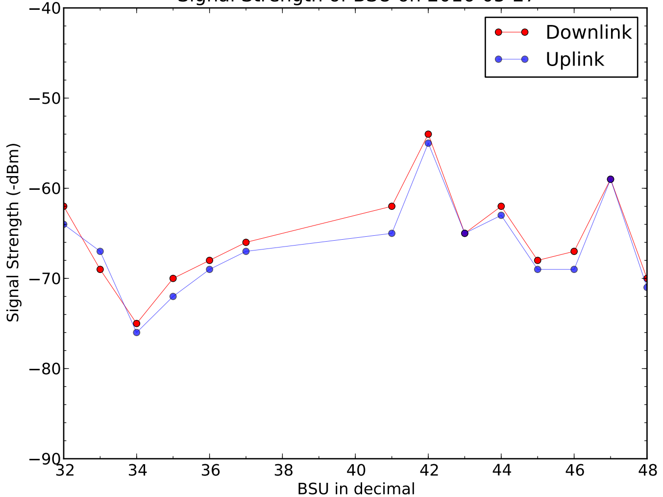
Signal Strength of BSU on 2016-05-27
