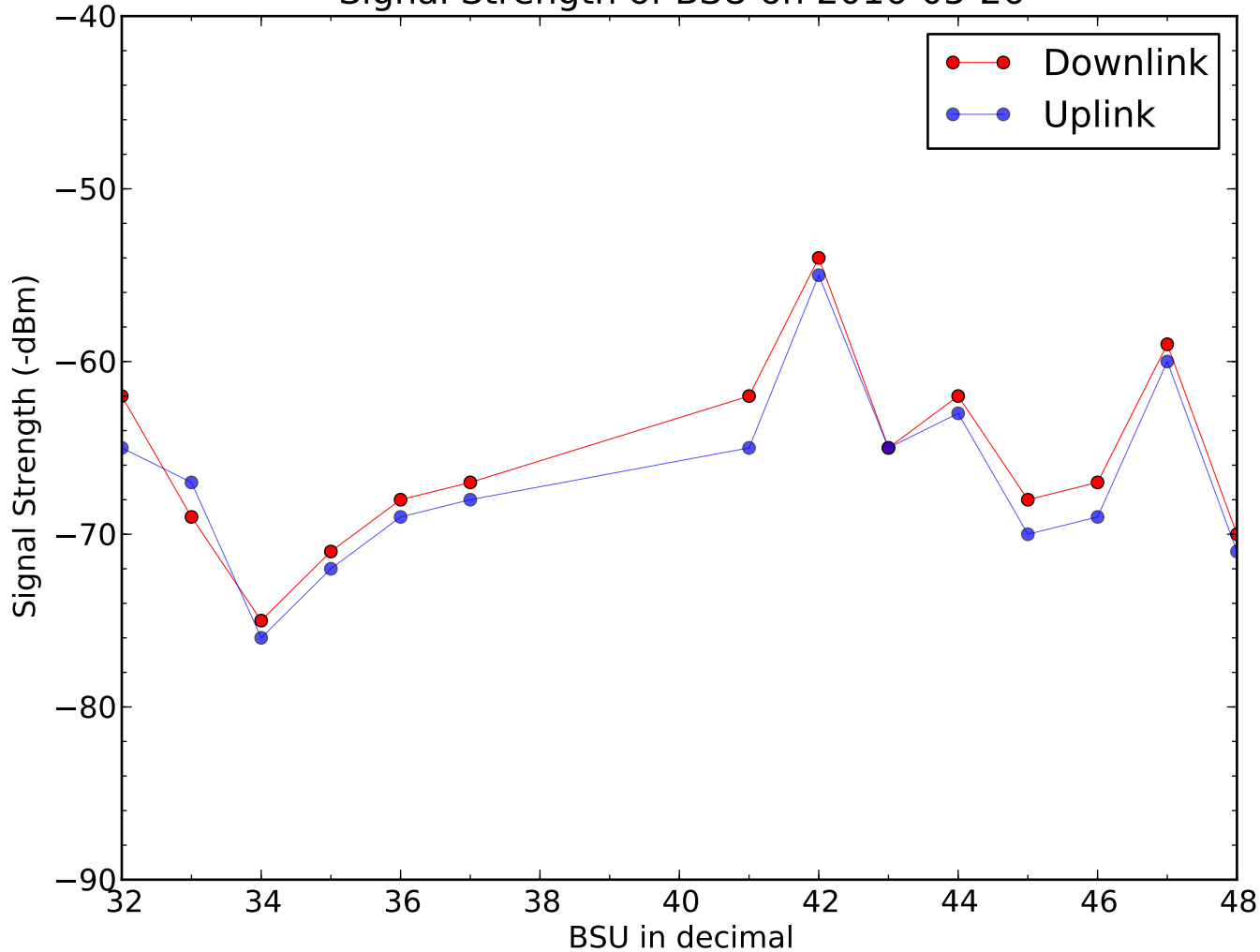
Signal Strength of BSU on 2016-05-26
