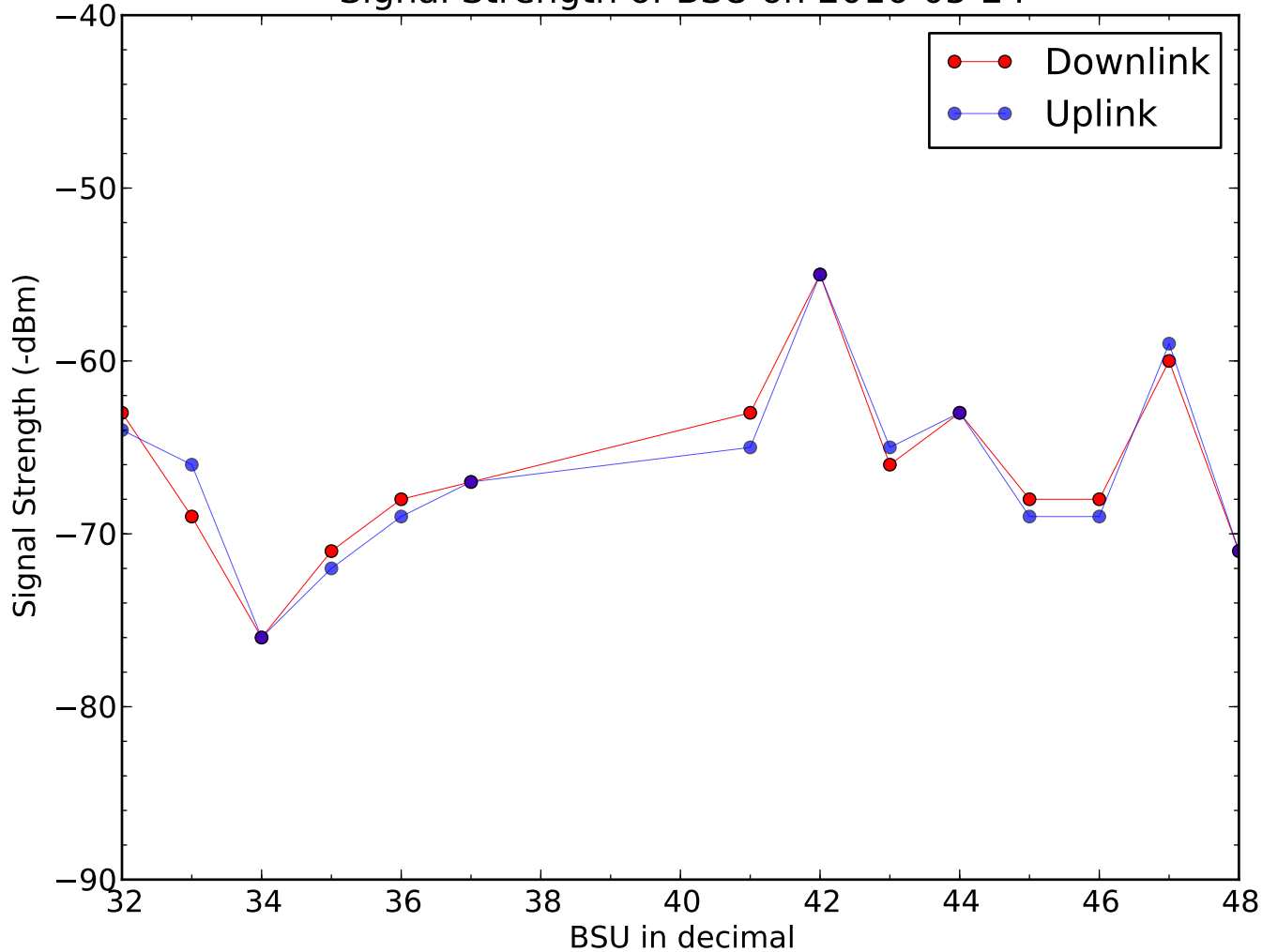
Signal Strength of BSU on 2016-05-24
