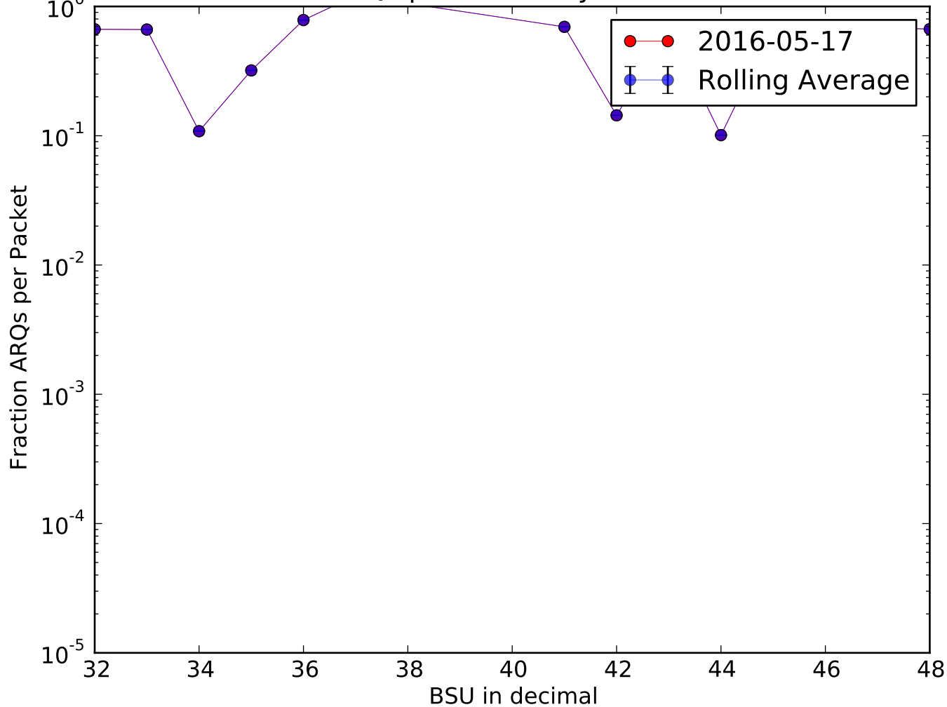
Fraction ARQs per Packet by BSU 2016-05-17
