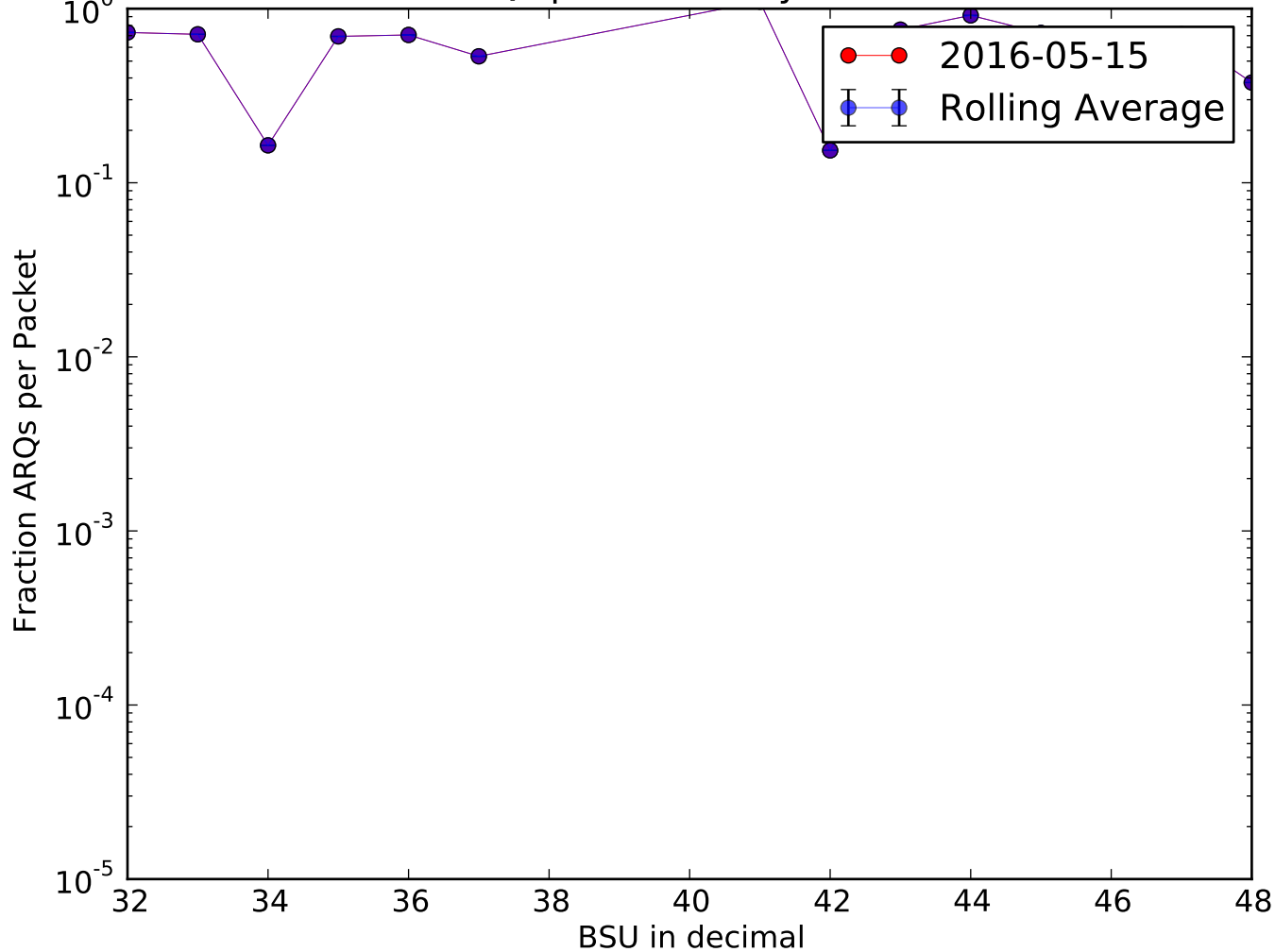
Fraction ARQs per Packet by BSU 2016-05-15
