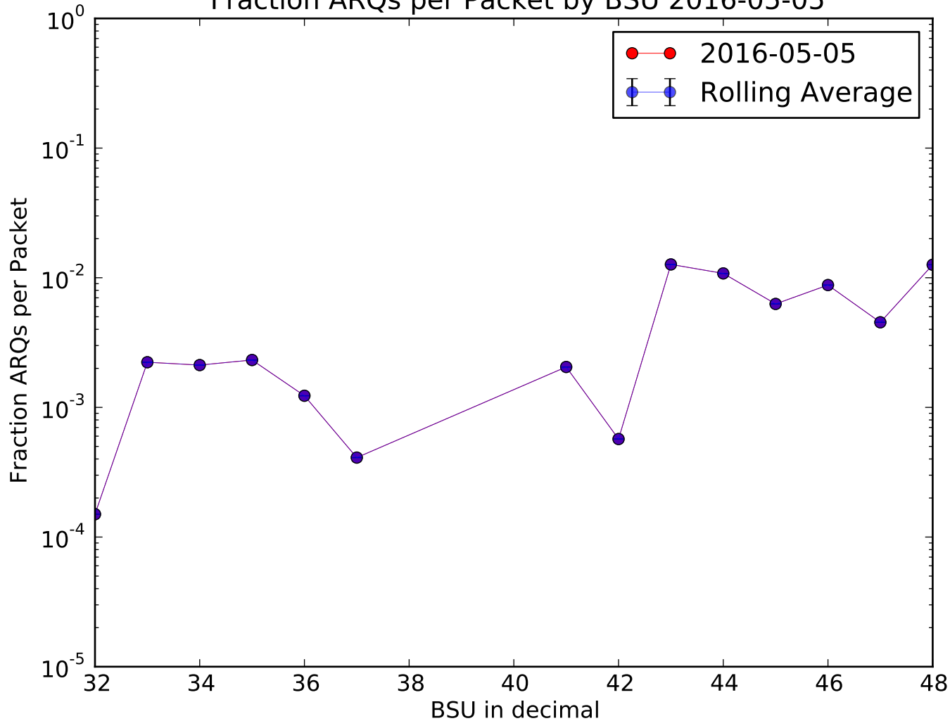
Fraction ARQs per Packet by BSU 2016-05-05
